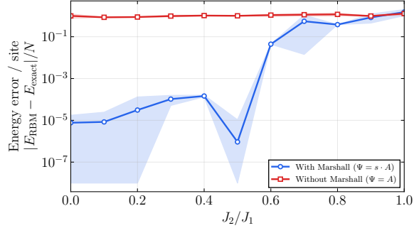
FIG. 11. Heisenberg energy error per spin, positive-amplitude vs. fixed-Marshall-sign ansatz, N = 8 , three seeds. Bands are recorded standard deviations.
