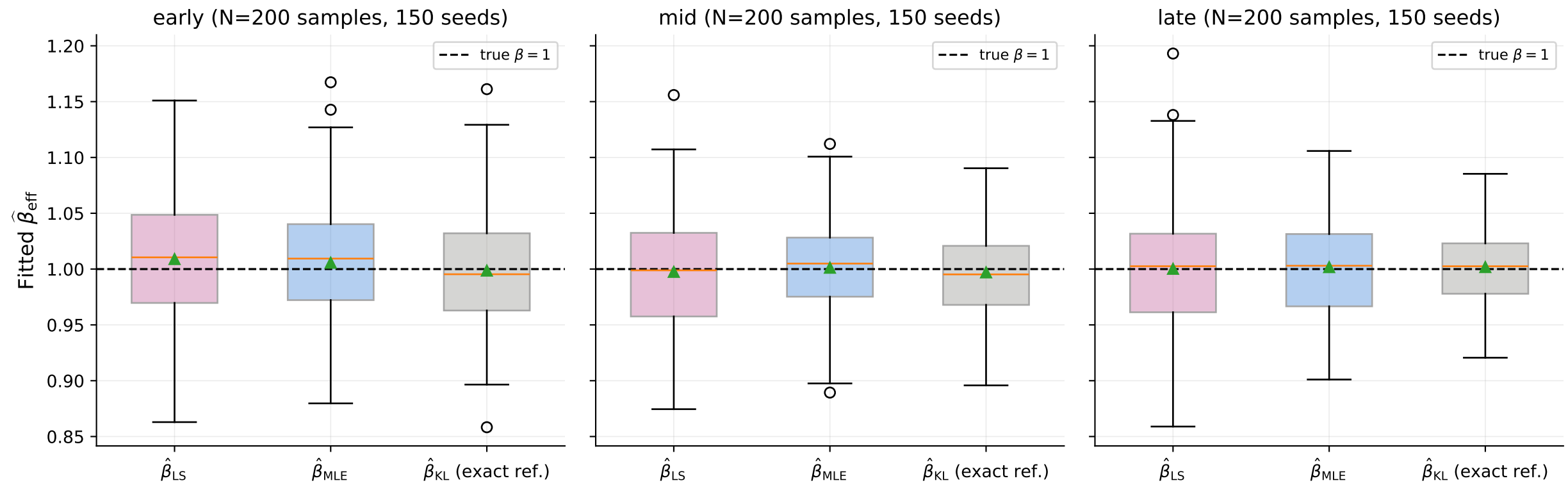
Conditional-MLE vs. least-squares \beta_{\text{eff}} : known-truth test ( N = 8 , h = 1.0 , Gibbs samples at exact \beta = 1 )
