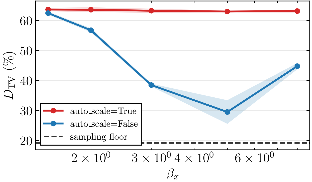
(a) Total variation distance D_{TV} between the QPU samples and |\Psi(v)|^2 .
