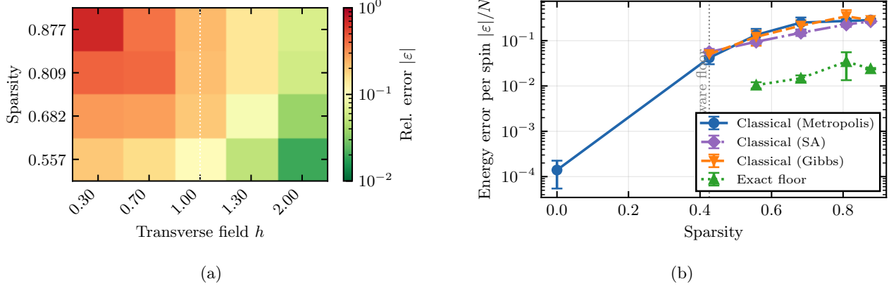
Figure 14: Error as a function of sparsity, with the number of hidden units kept equal to the number of visible units in both plots. (a) Error for different values of h , trained classically via Metropolis sampling. (b) Error at h = 1 across three classical samplers (Metropolis, simulated annealing, and persistent Gibbs), all using identical hyperparameters (300 SR iterations, learning rate 0.05), against the exact-ansatz floor, which uses noise-free gradients for up to 3000 iterations to escape optimization plateaus. The dotted line marks the exact-ansatz floor at this size. The vertical dashed grey line marks the native hardware floor: the sparsity of the unpruned chain-free embedding for this system size, i.e. the fraction of visible-hidden pairs with no real coupler between them before any edges are deliberately removed. All tested sparsity levels lie to its right, since pruning can only remove couplers, never add ones the chip does not have.
