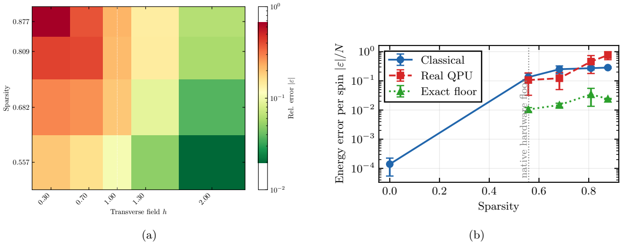
Figure 13: Error as a function of sparsity, with the number of hidden units kept equal to the number of visible units in both plots. (a) Error for different values of h . (b) Error at h = 1 , comparing classical training to training on the real QPU. The dotted line marks the exact-ansatz floor at this size.
