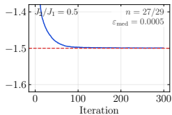
E/N vs. SR iteration, frustrated Heisenberg chain
