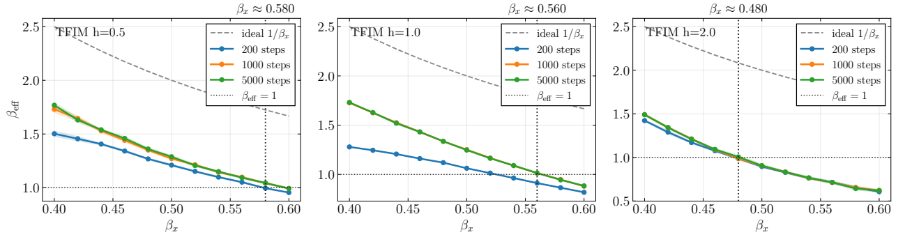
(b) Effective inverse temperature \beta_{eff} of the LSB samples, estimated by minimizing the total variational distance between the samples and the actual distribution. The dashed curve shows the ideal 1/\beta_x prediction for a perfect Gibbs sampler, the horizontal dotted line marks the VMC target \beta_{eff} = 1 .
