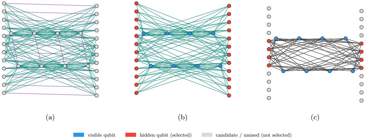
Figure 12: Construction of a chain-free sparse RBM from a D-Wave Zephyr hardware graph ( N = 8 visible units). (a) Identify internal couplers (green) and external/odd couplers (purple) (b) Creation of bipartite graph by restricting to internal couplers, splitting into hidden unit candidates (red) and visible units (blue). (c) RBM's visible-hidden connectivity mask by selecting the hidden units which maximize connectivity while keeping a min-set-cover. Non-selected candidates (grey) are dropped.
