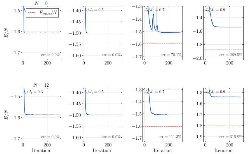
(b) Best RBM convergence curves ( E/N vs. SR iteration) for N \in \{8, 12\} and J_2/J_1 \in \{0.3, 0.5, 0.7, 0.9\} . The red dashed line marks the exact ground-state energy E_{\text{exact}}/N .
