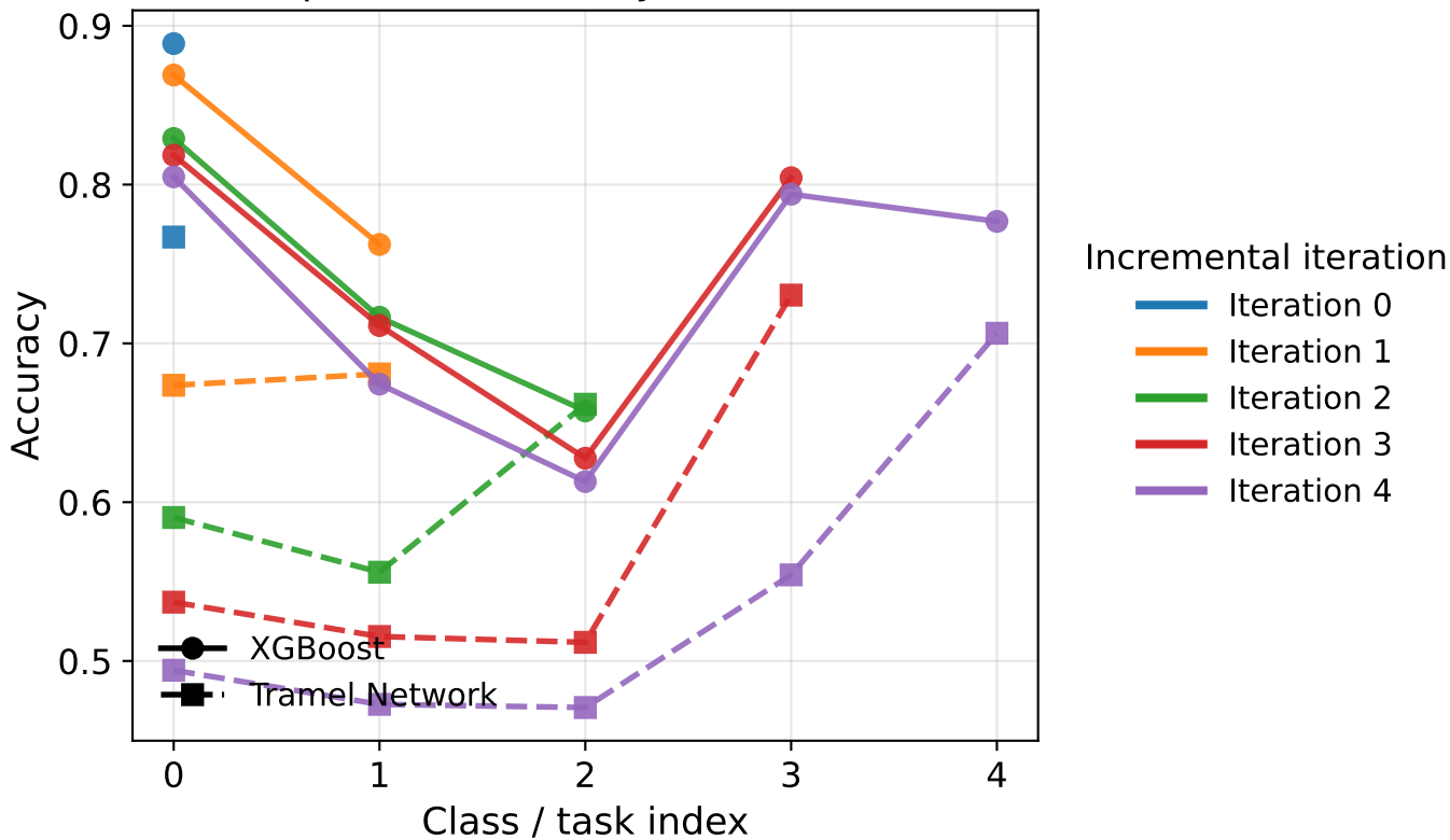
Per-class / per-task accuracy as tasks accumulate
