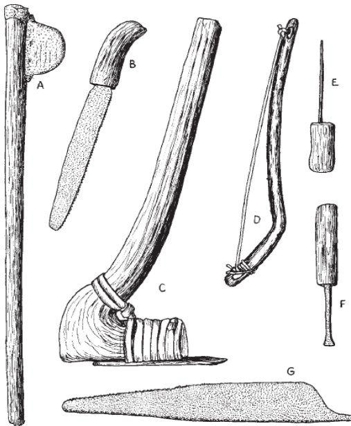
Carpenter's tools: (A) Bronze-headed axe. (B) Small handsaw with bronze blade. (C) Adze with bronze blade. (D) Wooden bow-drill. (E) Bit used with bow-drill. (F) Chisel. (G) Bronze saw blade. Note the minimal use of metal in these essential tools.
