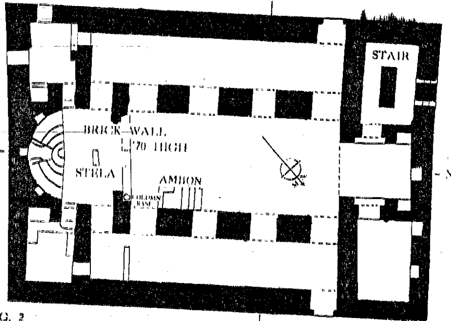
FIG. 2 GROUND PLAN SCALE 1/100
