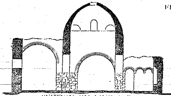
CHURCH NORTH OF KASR IBRÎM
