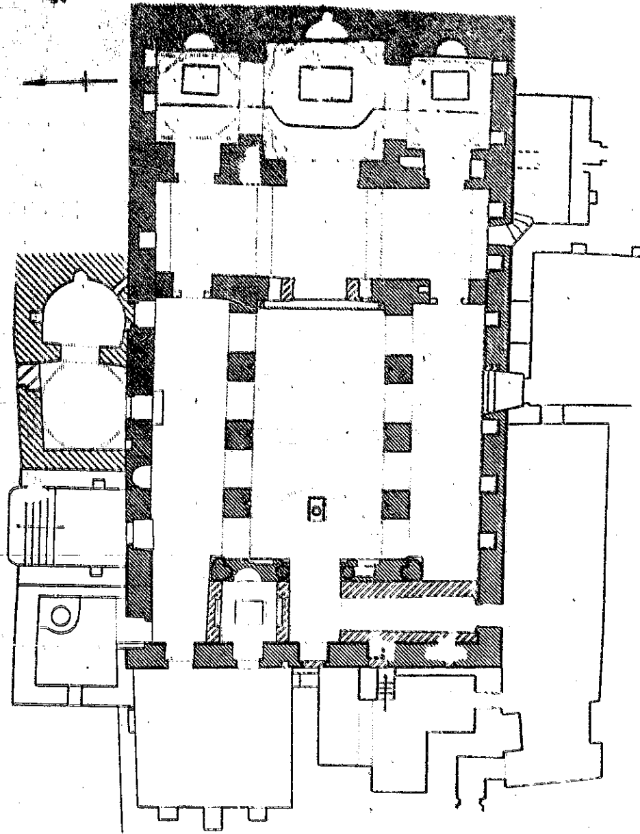
al-'Aqra' Dair al-Barmou
