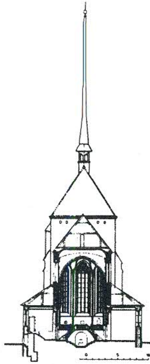
Cross-section of the Church of St. Verena in Zurzach
