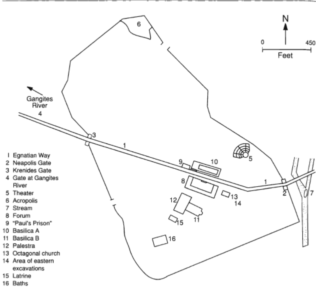
Schematic of Philippi
