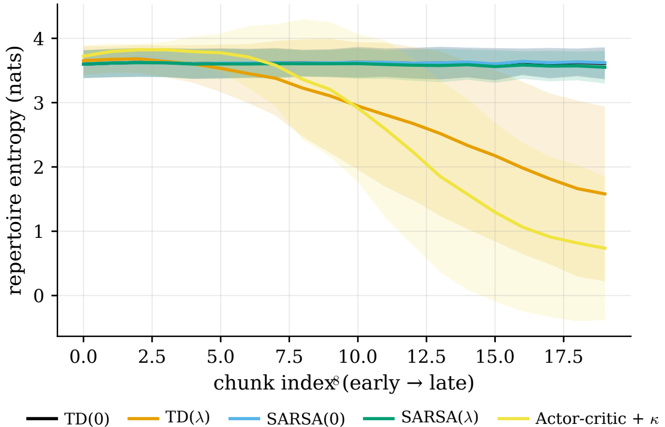
Figure 9. Repertoire entropy.
