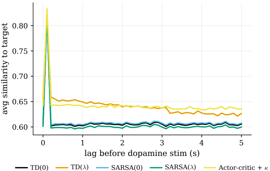
Credit kernel across lag (Tang paradigm replay)
