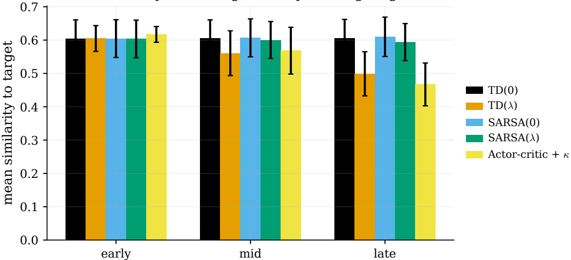
Similarity-narrowing curve by training stage
