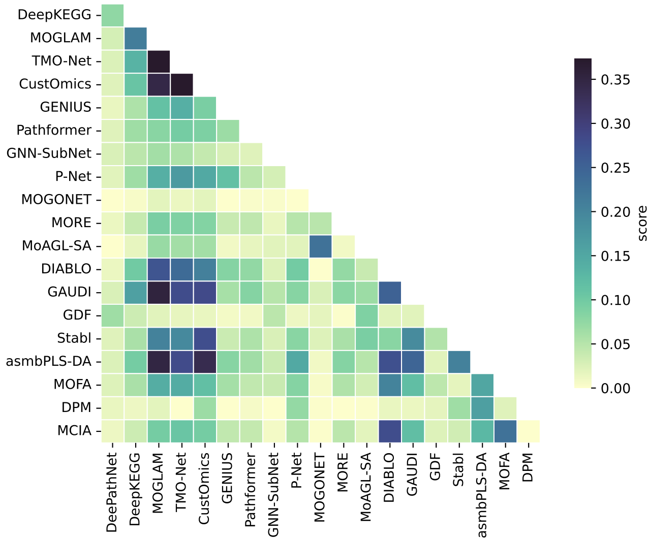
Methods ranking similarity (Kendall's \tau )
