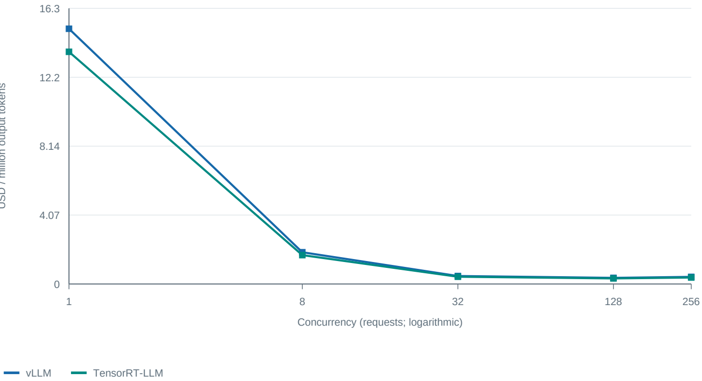
Long decode GPU unit cost
