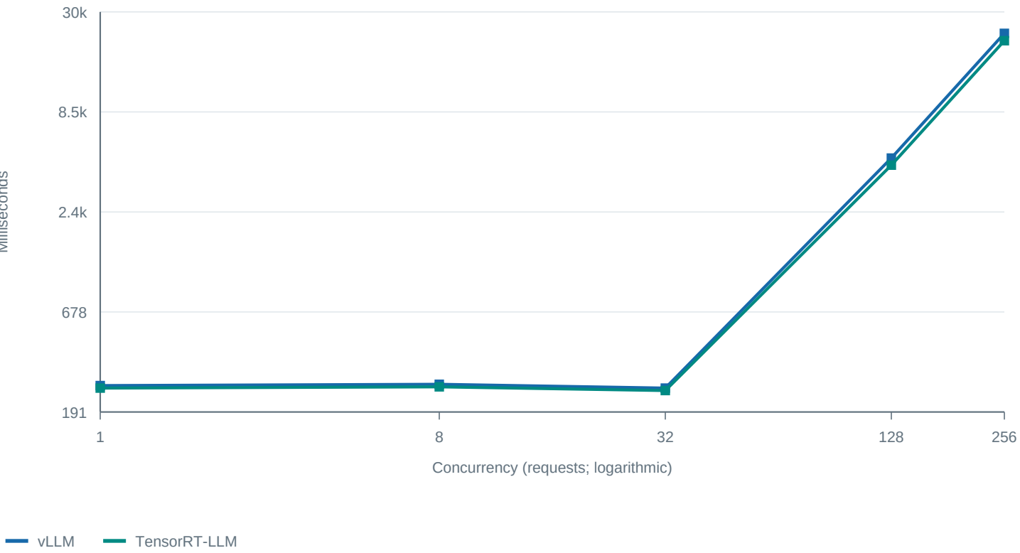
Mean run P95 TTFT: balanced
