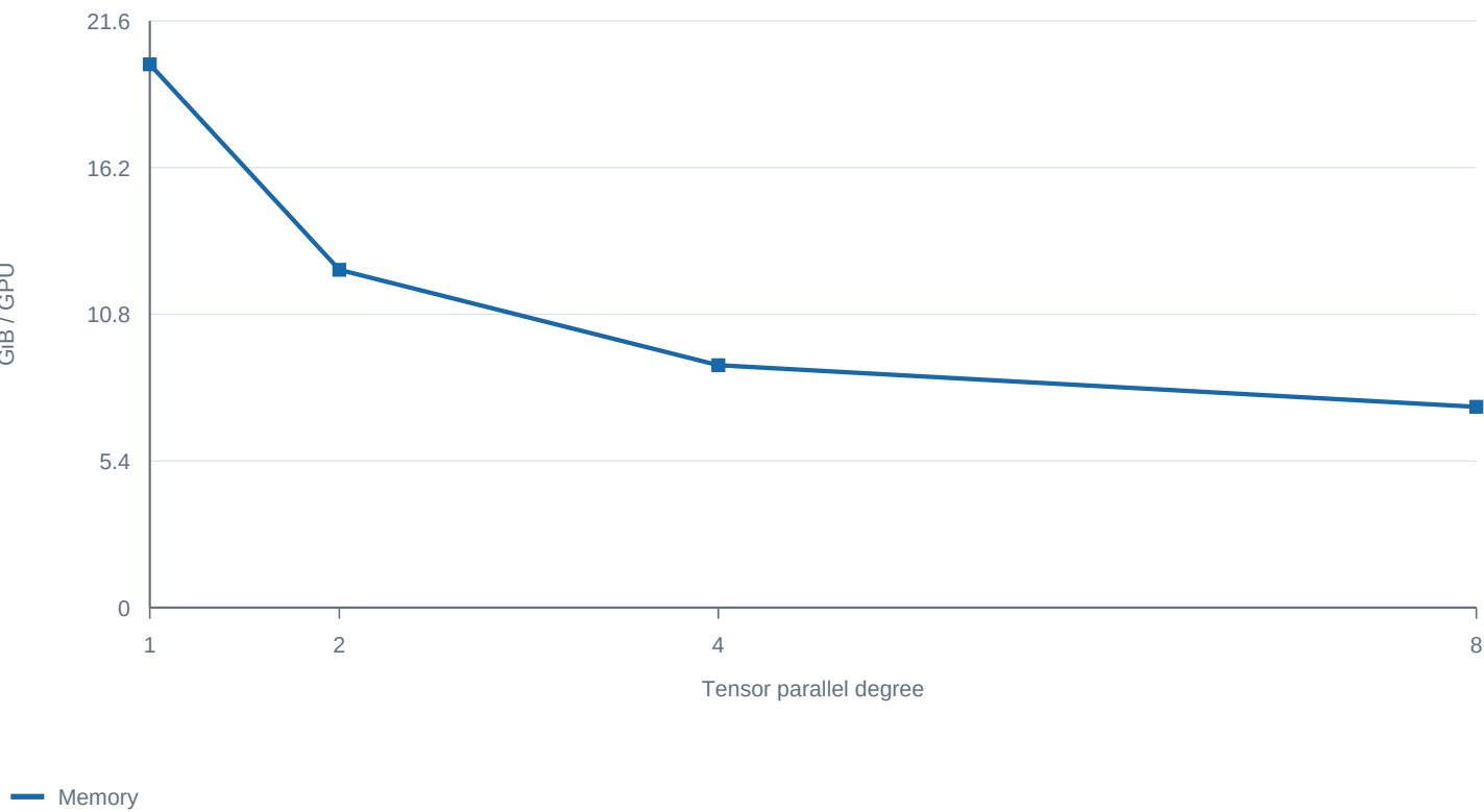
GPU memory at concurrency 32
