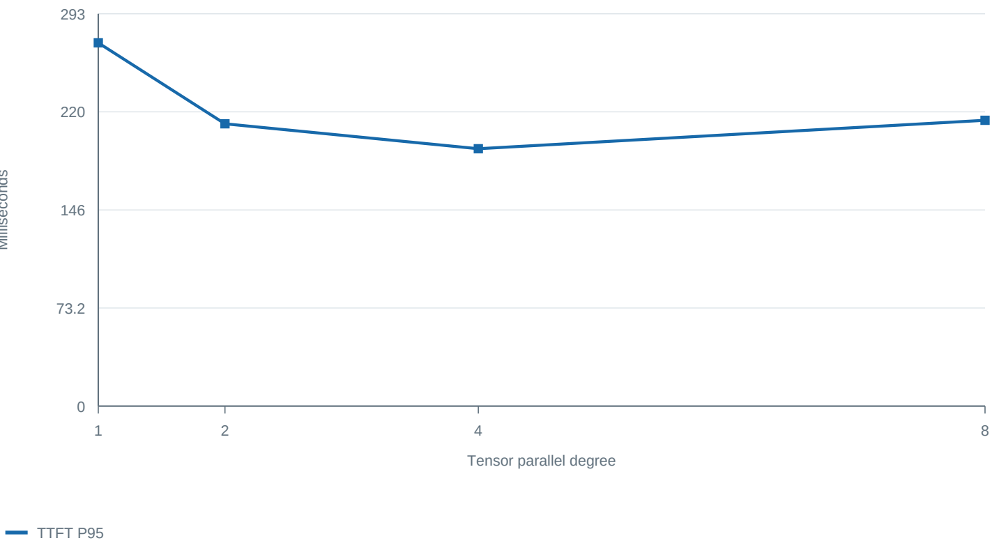
Mean run P95 TTFT at concurrency 1
