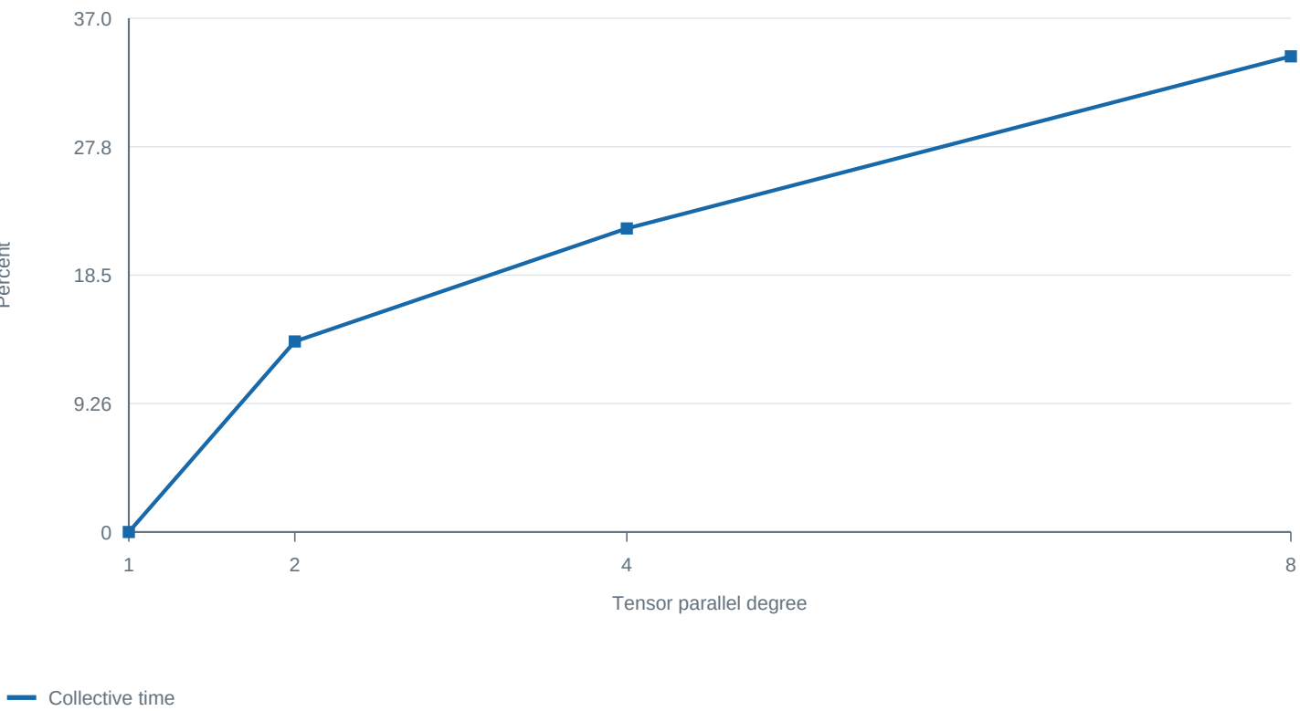
Collective time at concurrency 32
