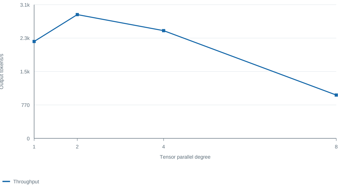
Output throughput at concurrency 32
