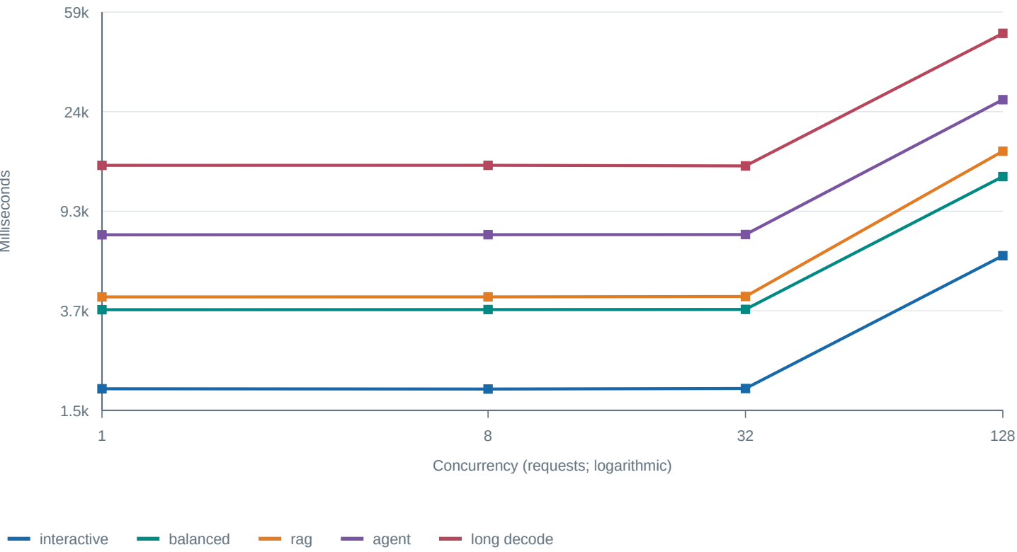
Mean run P95 end-to-end latency
