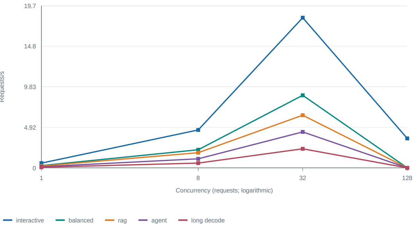
Joint SLO goodput
