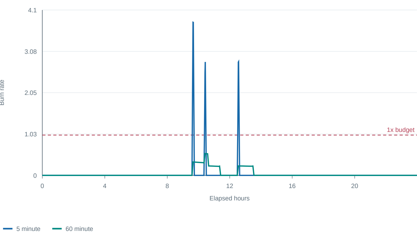
Latency error-budget burn
