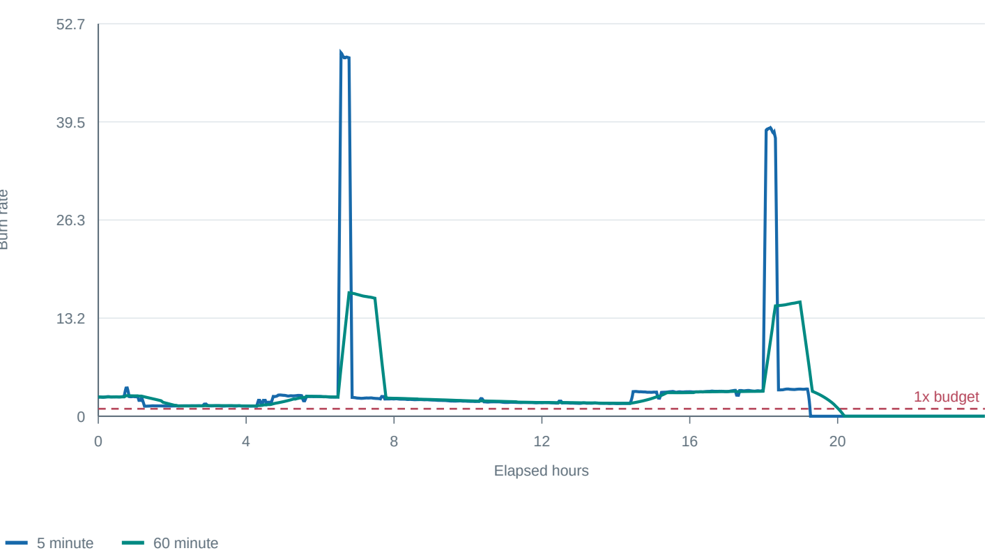
Availability error-budget burn
