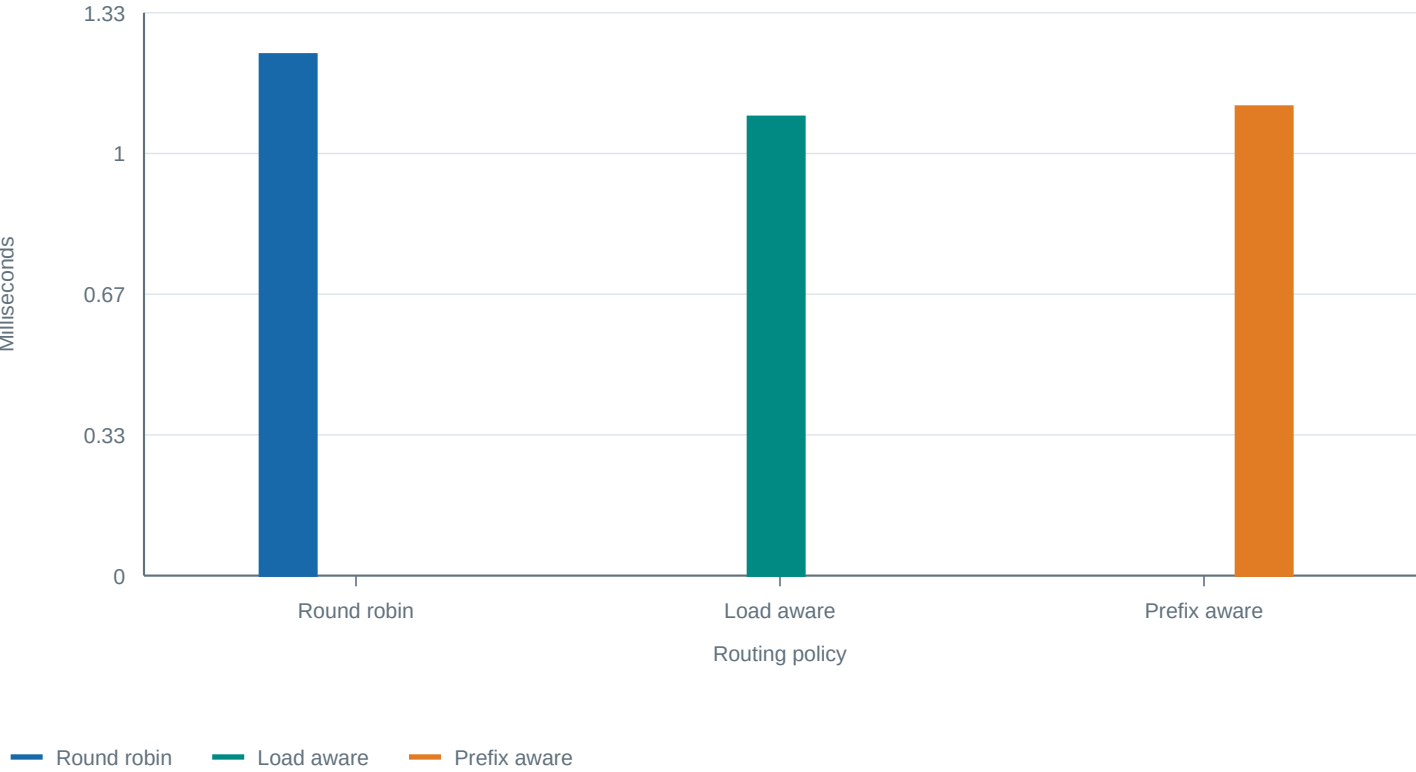
Mean run P95 queue latency
