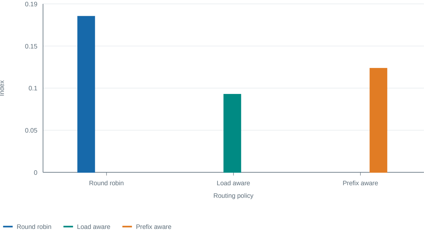
Worker load imbalance index
