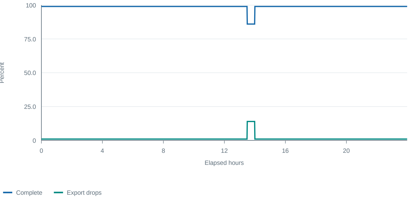
Trace delivery
