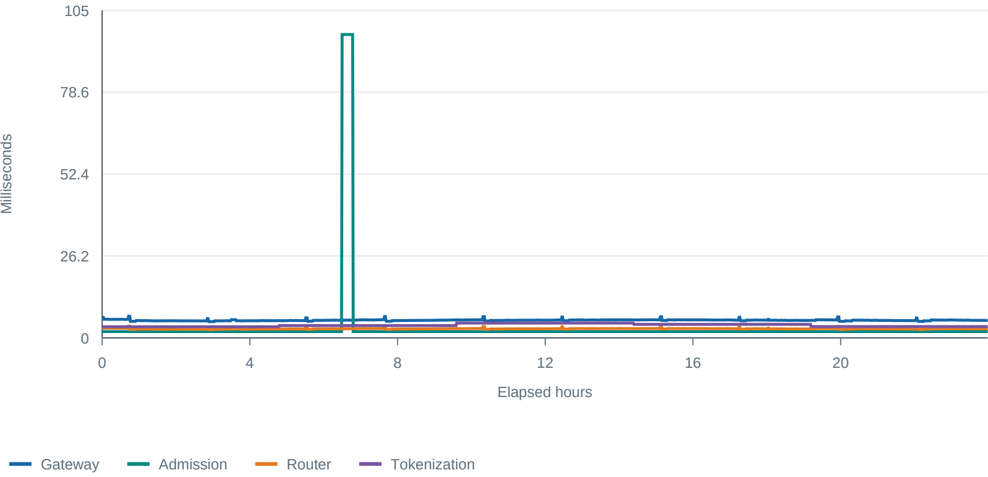
Request-path latency
