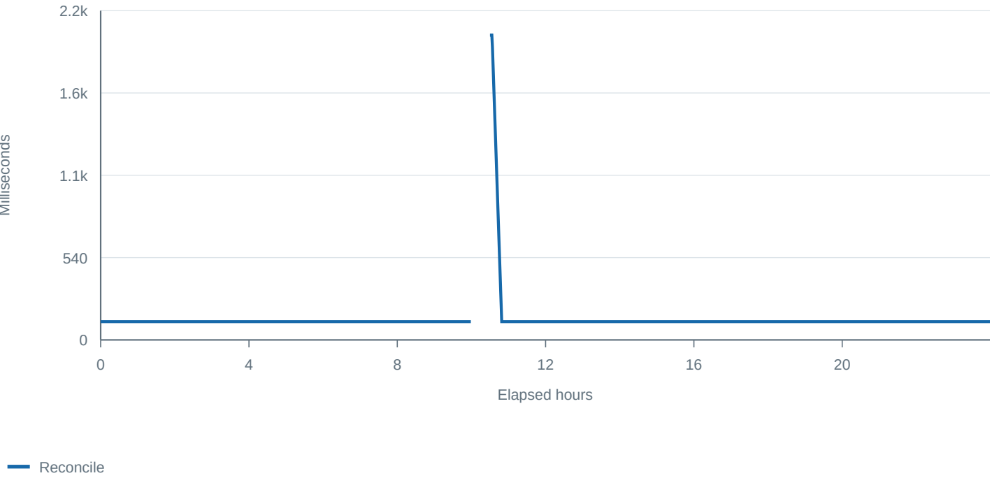
Reconcile latency
