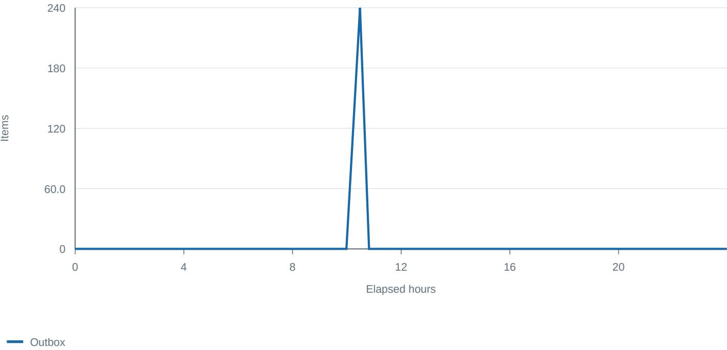
Outbox backlog
