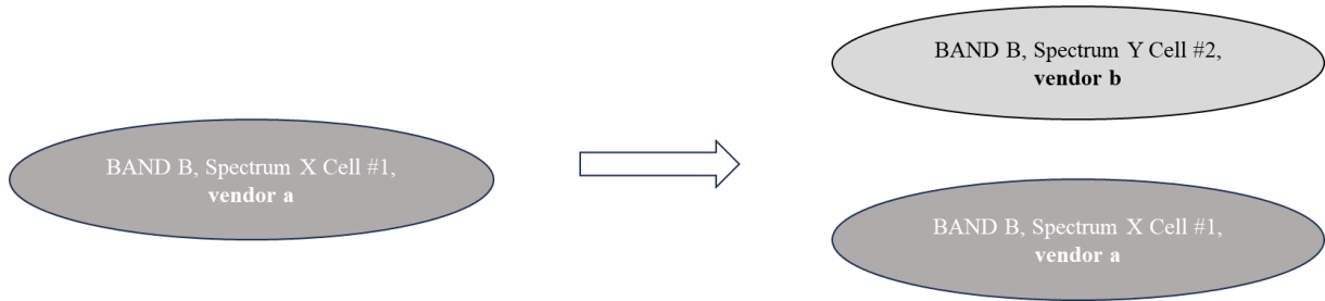
Figure 5.3.2.5-1: Example of spectrum aggregation in intra band contiguous and non-contiguous spectrum
