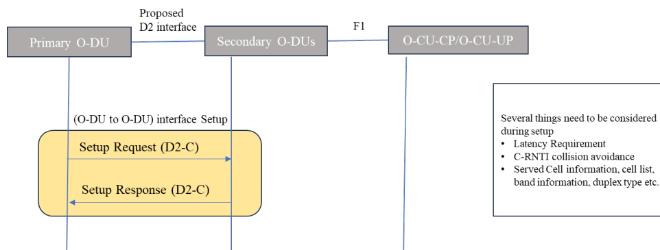
Figure 6.3.1-8: D2 link establishment.
