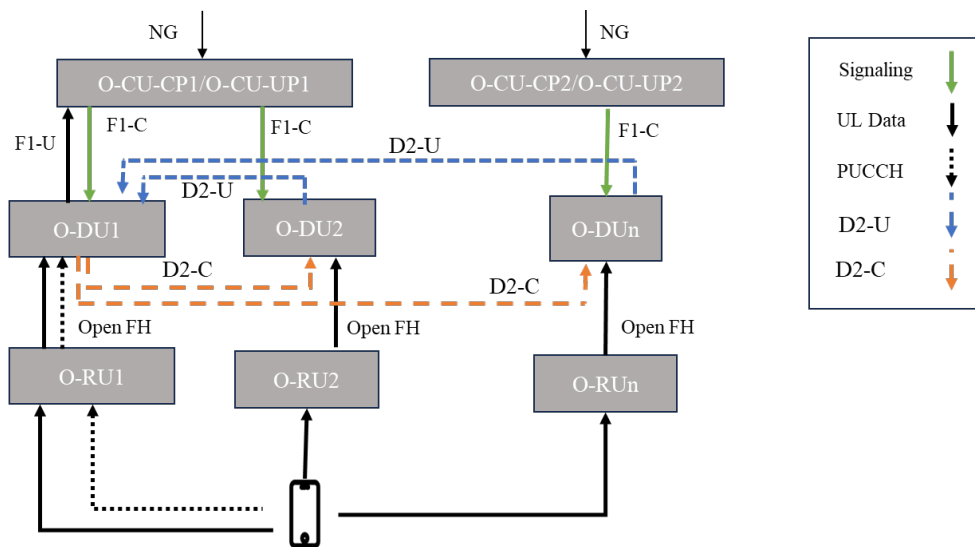
Figure 6.3.1-3: Inter O-DU UL CA, PUCCH on PCell.
