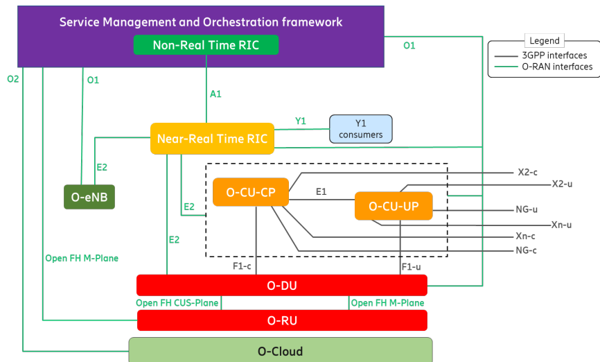
Figure A.4-3: Aggregated O-CU-CP, O-CU-UP, and O-DU
