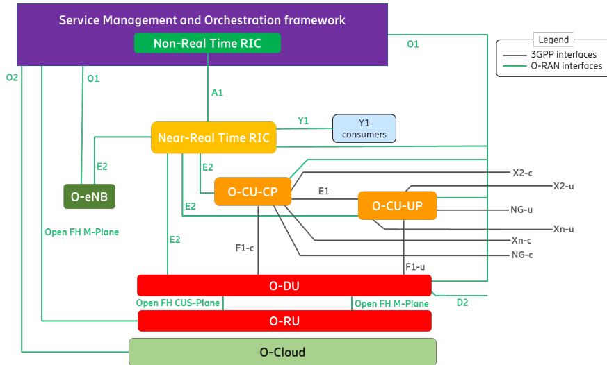
Figure A.4-1: Disaggregated O-RAN Network Functions
