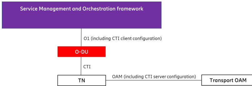
A.5-1: Simplified CTI Architecture
