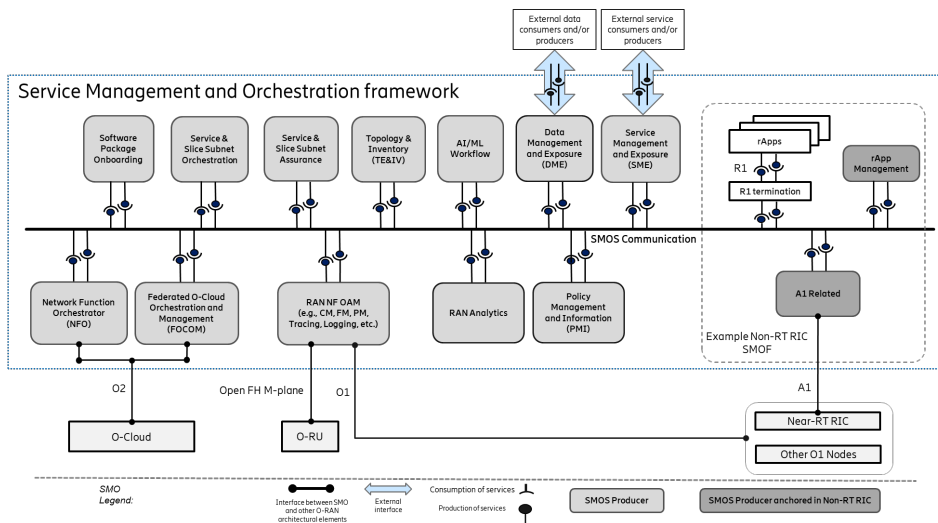
Figure 5.3.1.2.1-1: SMOSs in the SMO SBA representation
