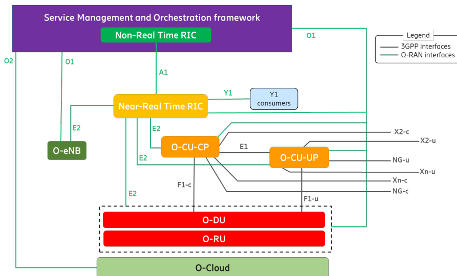
Figure A.4-6: Aggregated O-DU and O-RU
