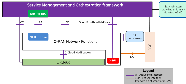
Figure 5.1-1: High Level Architecture of O-RAN
