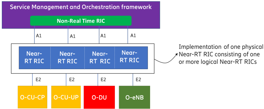
Figure A.3-2: Distributed Near-RT RIC
