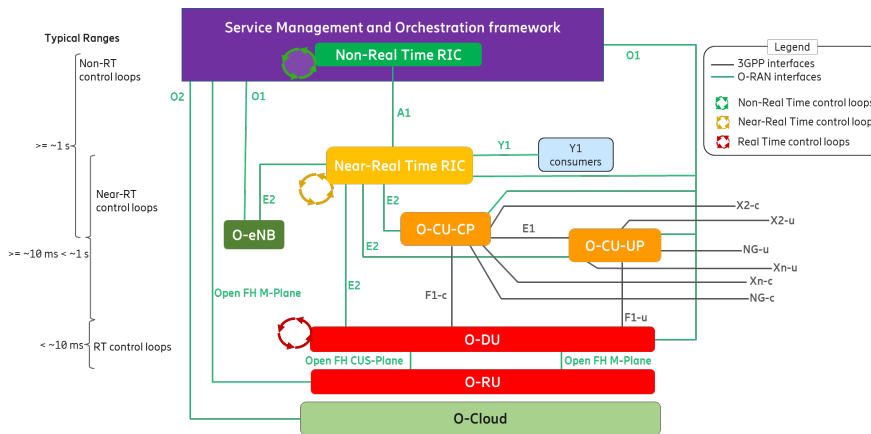
Figure 5.2-1: O-RAN Control Loops
