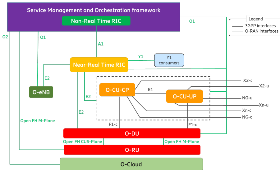
Figure A.4-2: Aggregated O-CU-CP and O-CU-UP
