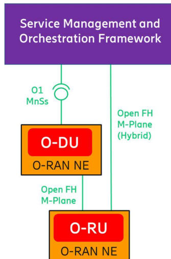
Figure 5.3.2-3 O-RAN Logical OAM Architecture, Hybrid M-Plane
