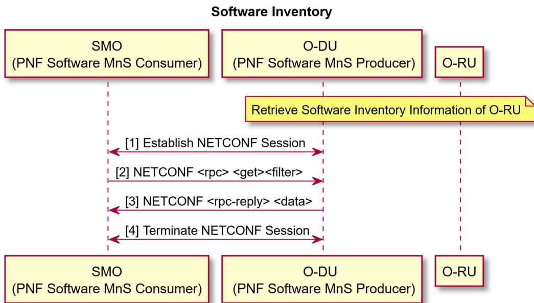
Figure 4.2.4.1.1.2-1: Software Inventory
