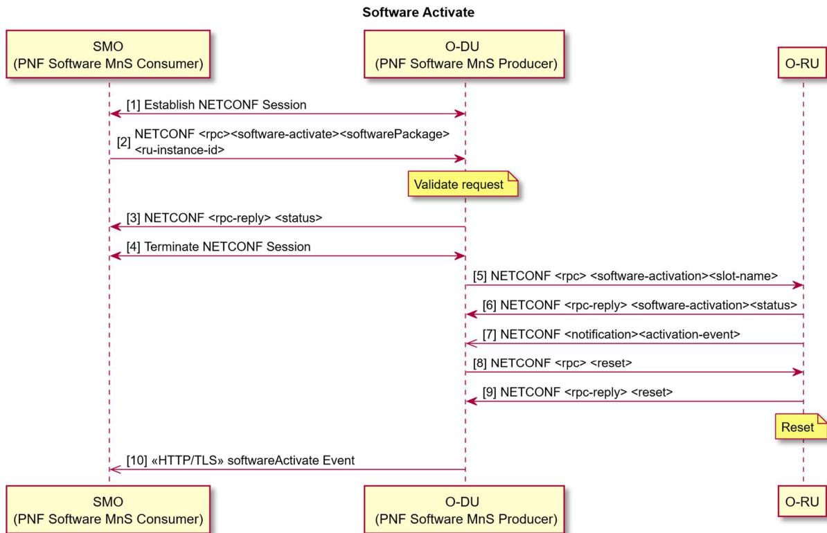
Figure 4.2.4.1.3.2-1: Software Activate
