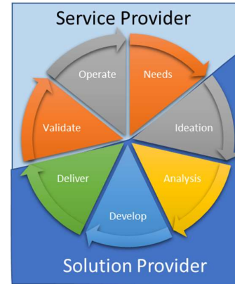
Figure 6-1: Generalized Lifecycle
