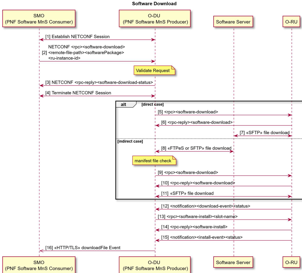
Figure 4.2.4.1.2.2-1: Software Download
