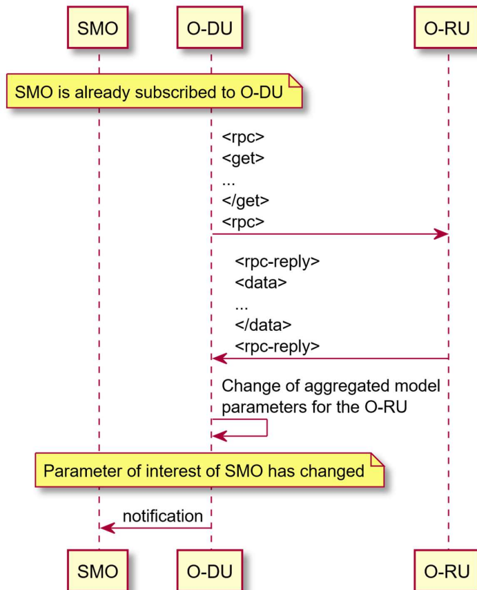
Figure 4.2.4.4.3.2-2: Notification to the SMO preceded by the O-DU <get> operation
