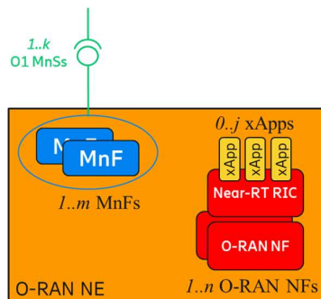
Figure 5.3.2-4 O-RAN Logical Network Element
