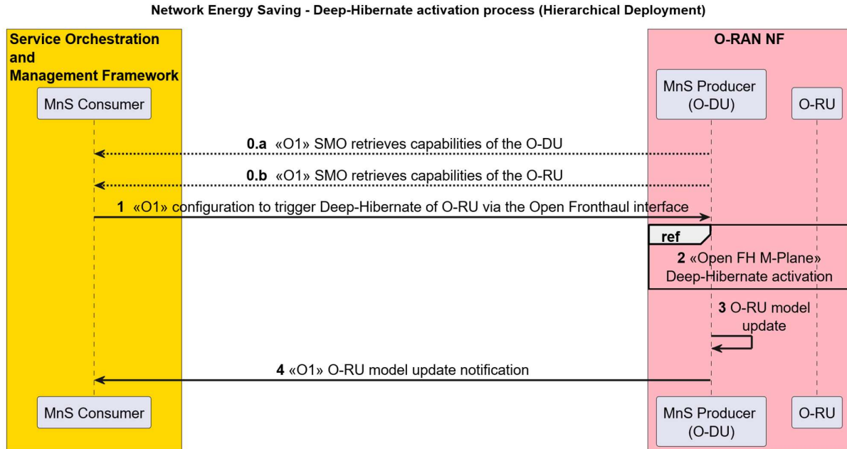
Figure 4.2.5.3.3-1: Deep Hibernate based Network energy saving activation using O1 interface
