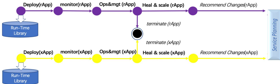
Figure 6.1.4.1-1: Service Provider Runtime Lifecycles
