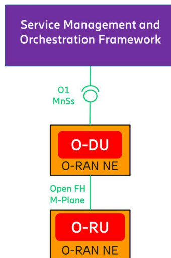
Figure 5.3.2-2 O-RAN Logical OAM Architecture, Hierarchical M-Plane
