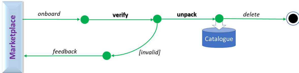
Figure 6.1.3.1-1: Onboarded AppPackage Service Provider Configuration Lifecycle
