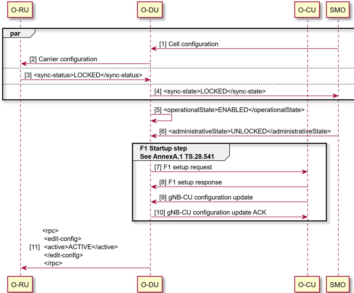
Figure 4.2.4.4.2.2-1: Cell activation procedure
