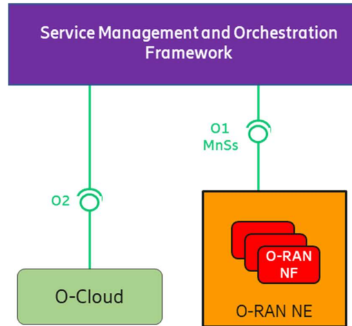
Figure 5.3.2-1 O-RAN Logical OAM Architecture, O1 and O2 Interfaces
