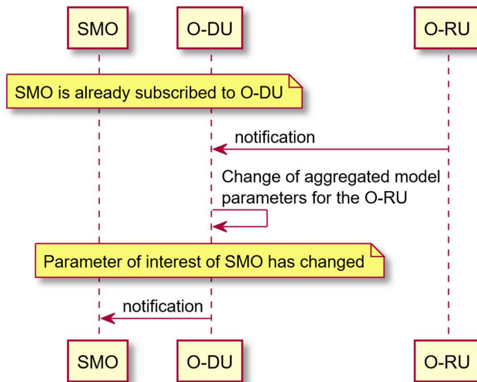
Figure 4.2.4.4.3.2-1: Notification to the SMO preceded by the O-RU notification
