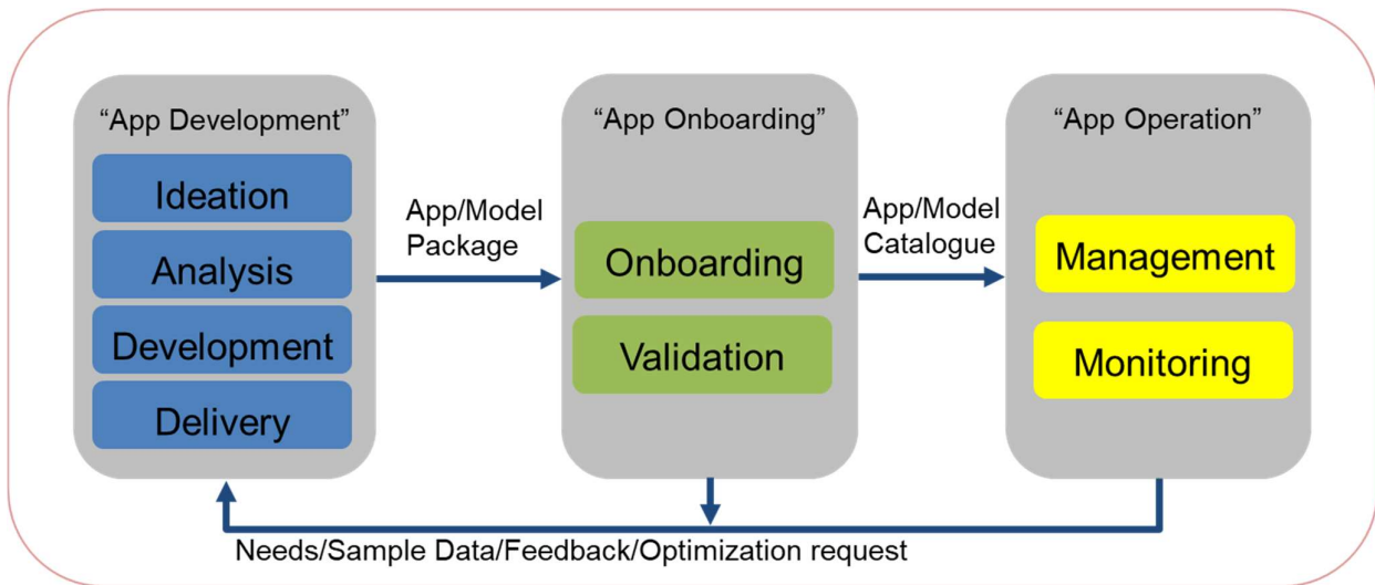
Figure 6.1-1 Application Lifecycle Phases
