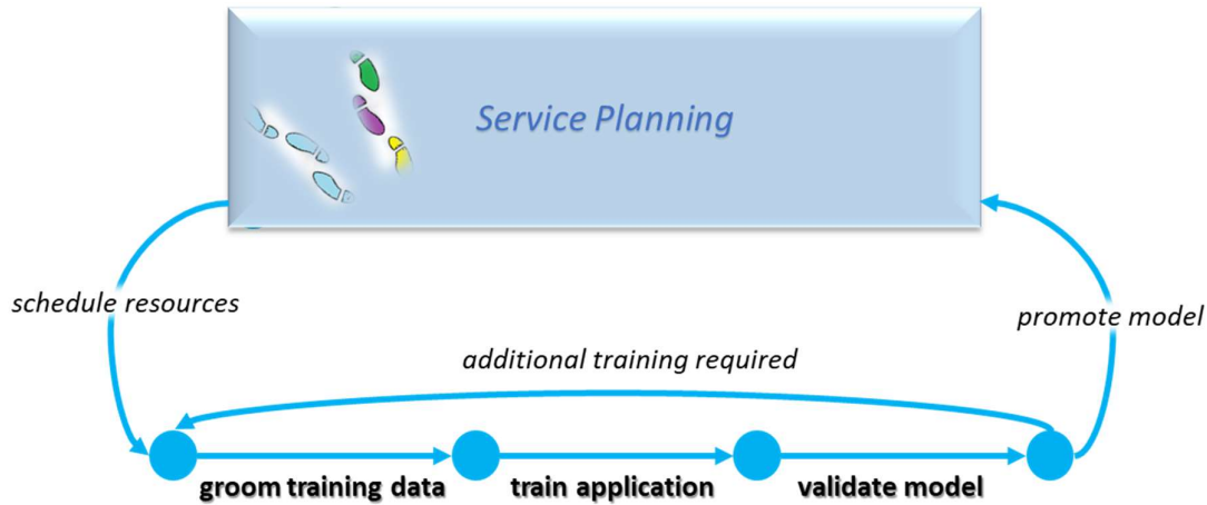
Figure 6.1.3.2.2-1: Training App Service Provider Training Lifecycle
