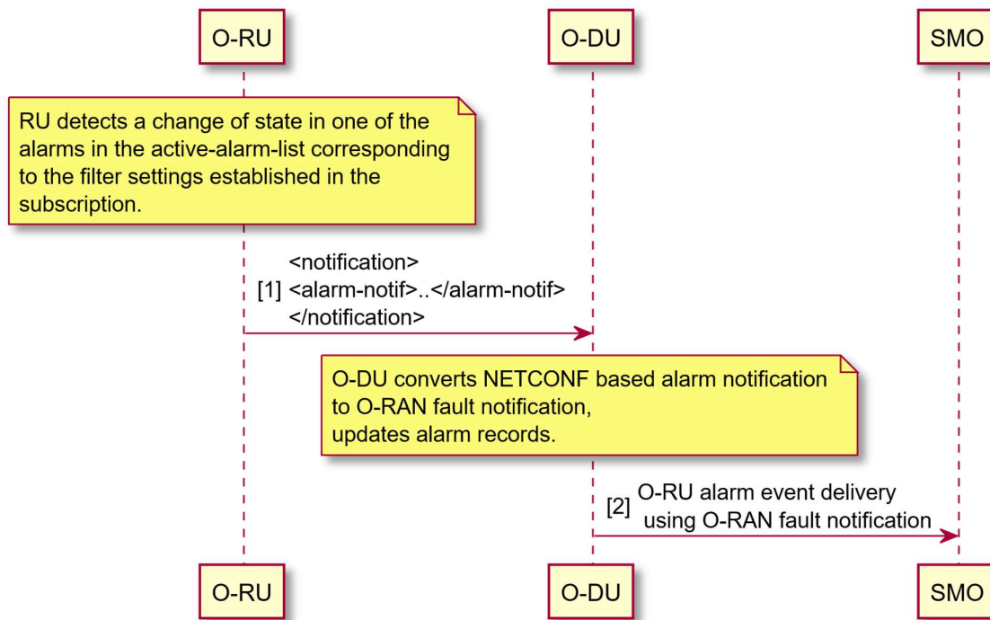
Figure 4.2.4.3.2-1: Operation to merge O-RU Alarms by O-DU
