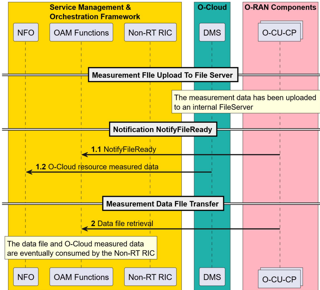
Figure 4.2.2.3.2-1: Measurement Data File Consumption
