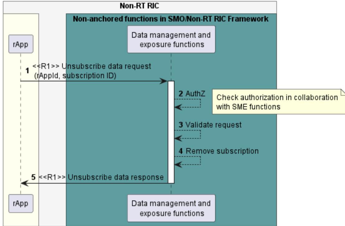
Figure 7.7.4.2-1: Terminate data subscription use case flow diagram.
