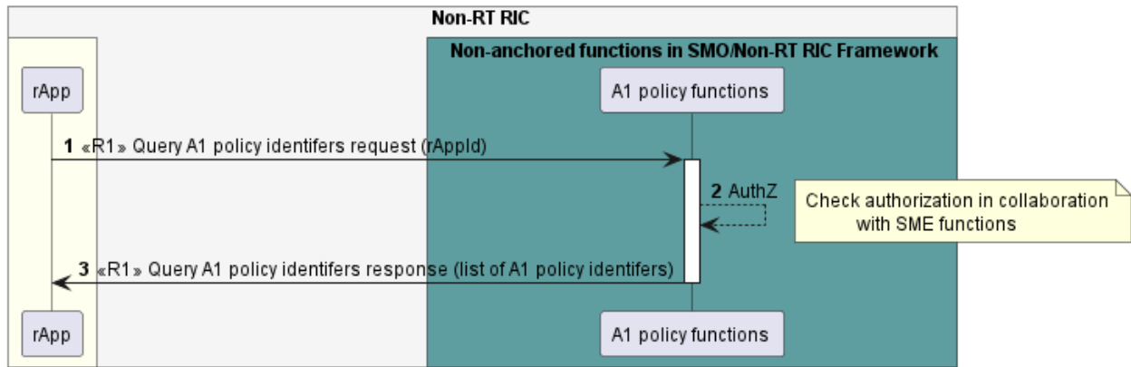
Figure 10.5.4.1-1: Query A1 policy identifiers use case flow diagram.
