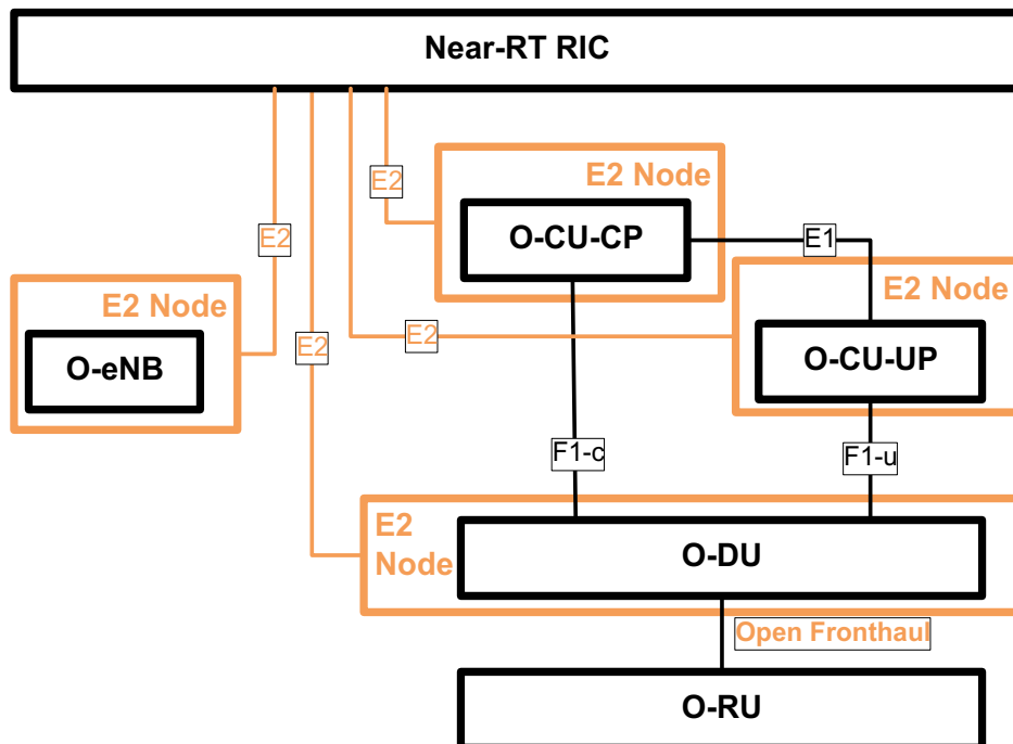
Figure 4.2-1: O-RAN architecture overview showing Near-RT RIC interfaces
