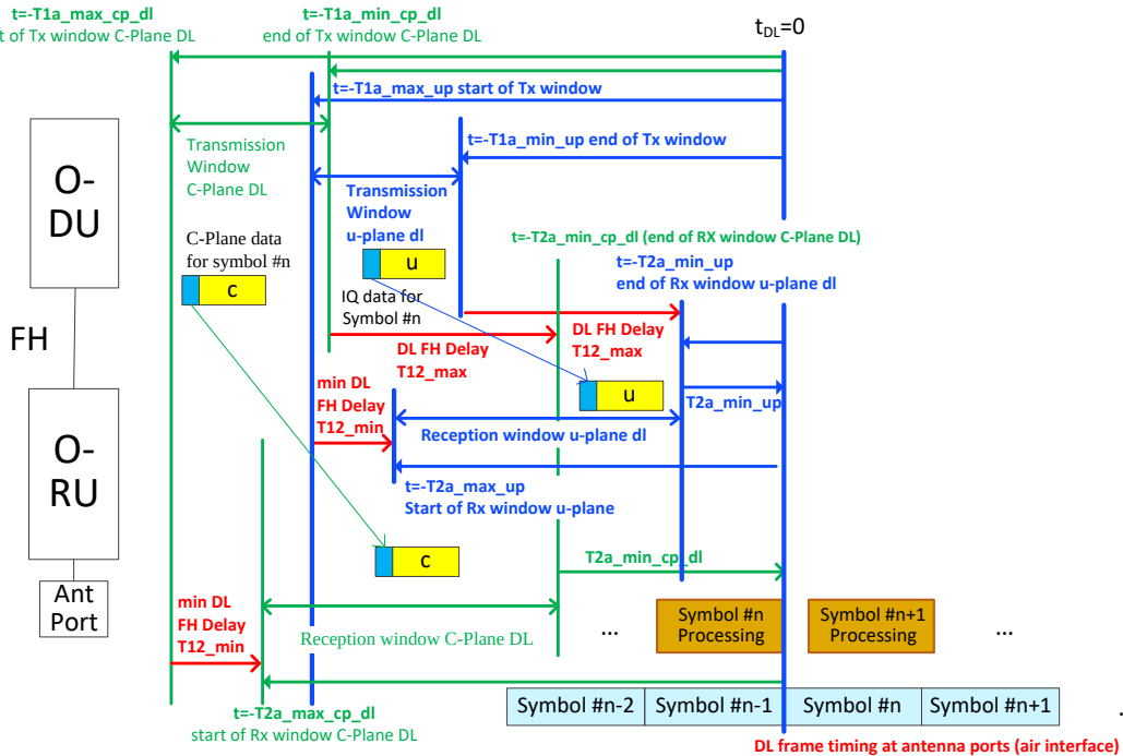
Figure B.1-2: Timing relations per symbol IQ in DL direction (U-Plane and C-Plane)
