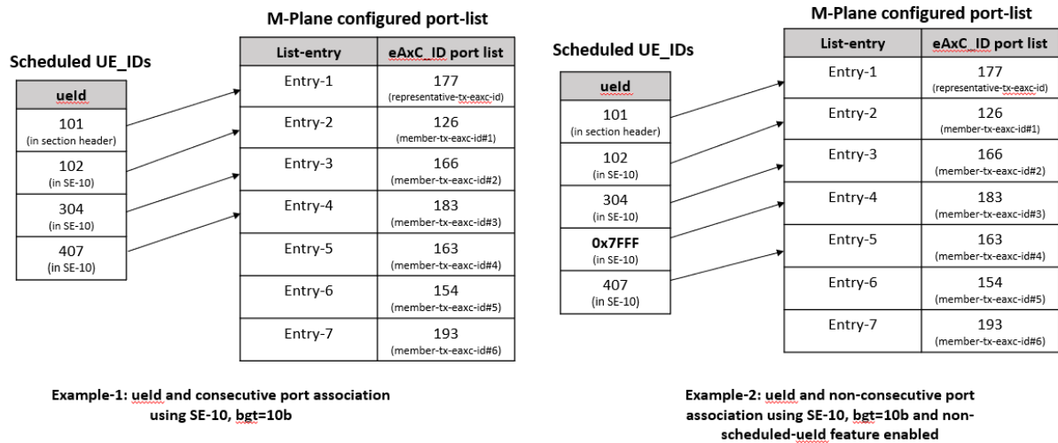
Figure 7.9.3.2-1 Consecutive and non-consecutive ports scheduled using beamGroupType=10b
