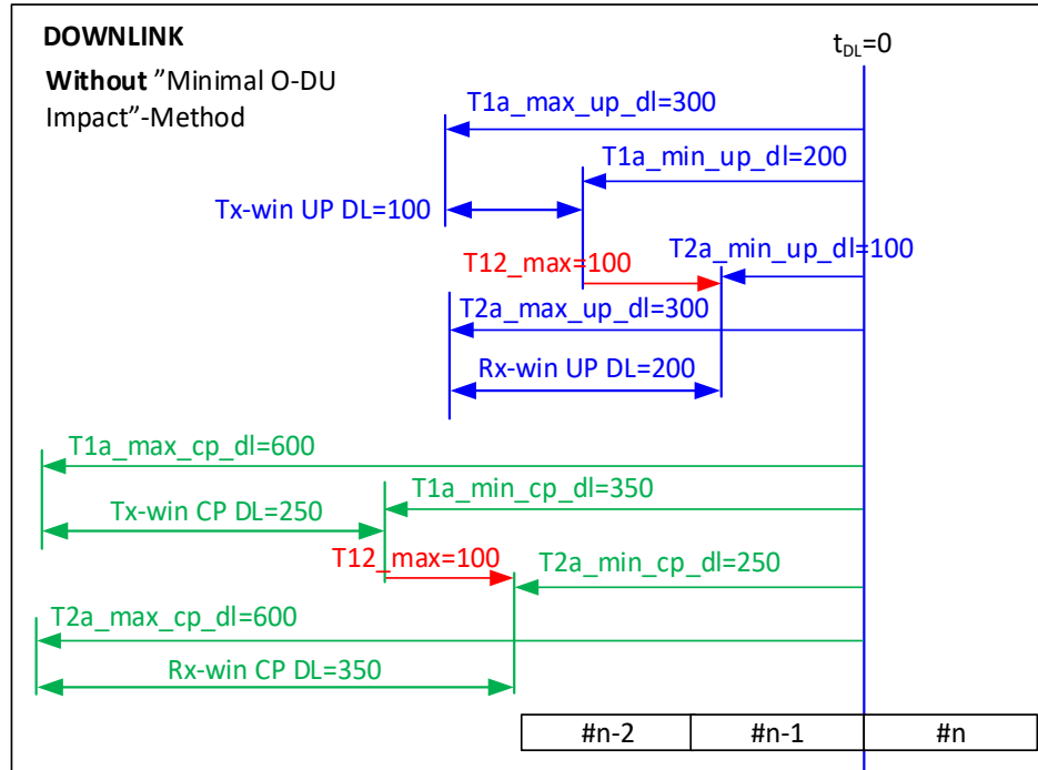
Figure 4.7.2.2-1: Downlink without using minimal O-DU impact method
