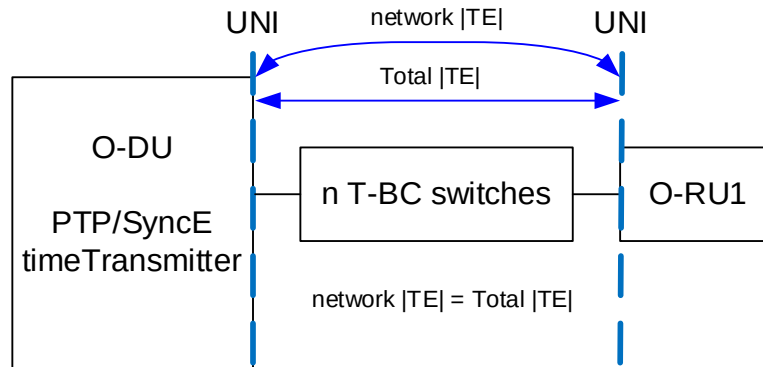
Figure H.2.3-2: Clock chain model for analysis
