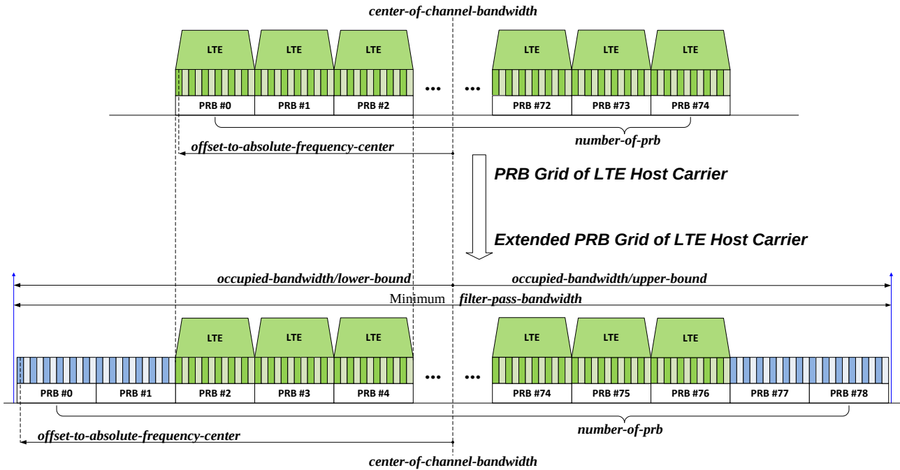
Figure 15.2.1-1: Example of extended PRB grid (DL)
