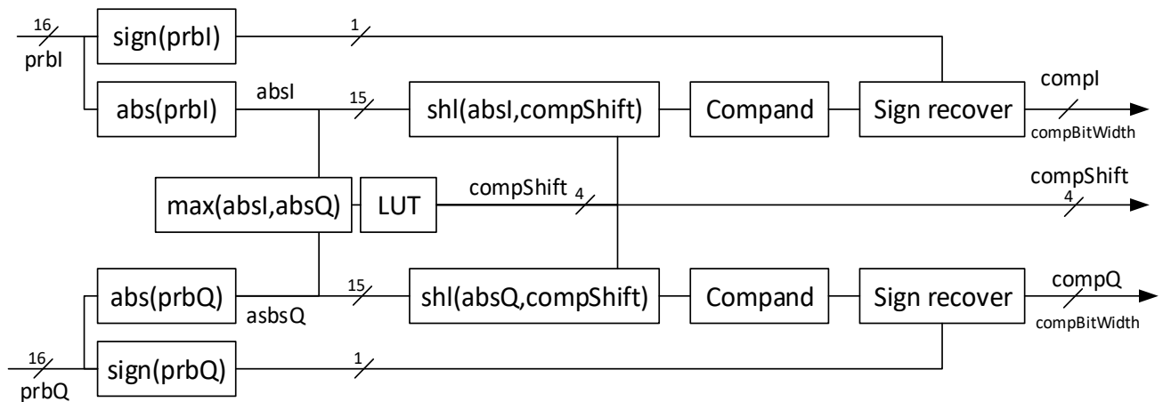
Figure A.3.1-1: \mu -Law compression algorithm
