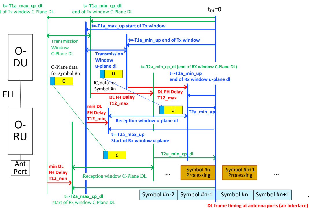
Figure 4.4.3-1: Timing relations per symbol IQ in DL direction (U-Plane and C-Plane)
