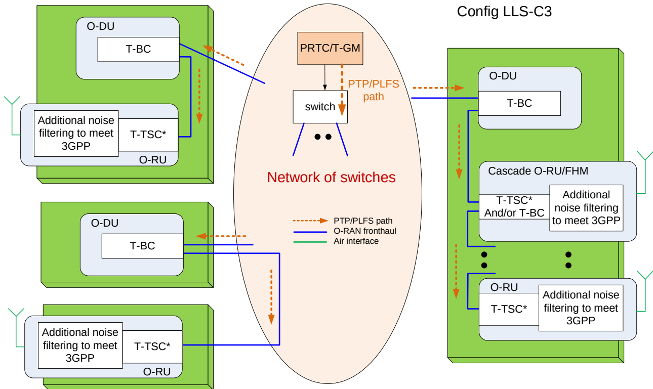
Figure 11.2.2.3-2: Example of configuration LLS-C3 synchronization (O-DU clock part of the synchronization chain from PRTC to the O-RU)
