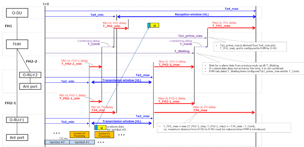
Figure 13.5.3-1: Delay model parameters for FHM mode (2 O-RUs case, i.e. N_m=2 , is illustrated as an example)
