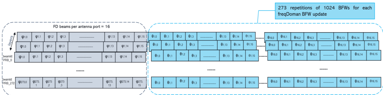
Figure 12.4.3.4.4-2: Example of repetition of time-domain beamforming weight vector of size K' * numAntElements for every frequency-domain beamforming update (per prb per layer)
