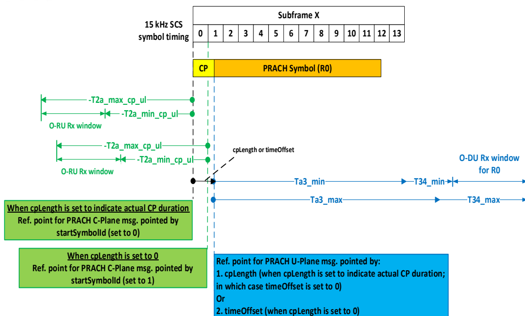
Figure 4.4.3-3: Timing relations for PRACH (Example 1: PRACH Format 0)
