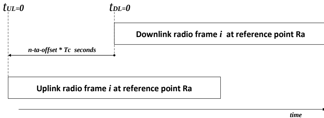
Figure 4.8.1-1 : Uplink-Downlink Timing Relation
