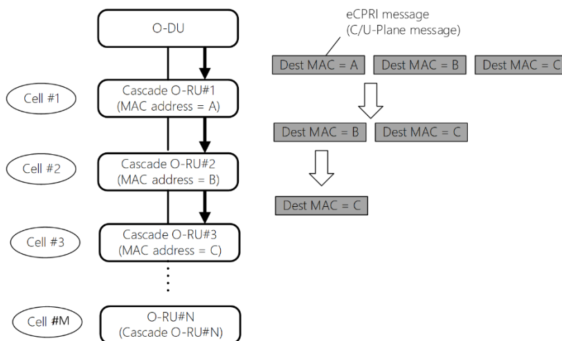
Figure 13.4.2-1: Downlink flow for Multiple Cell scenario
