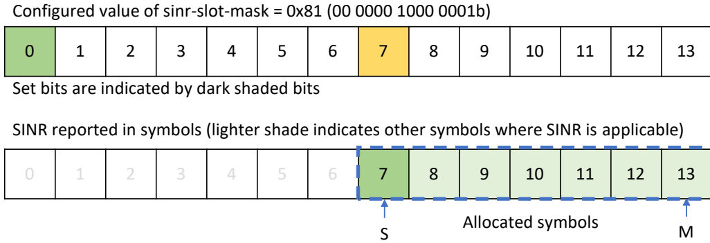
Figure 7.2.11-2: Example 5 of SINR reporting in Section Type 9 with \text{sinr-slot-mask} = 0x81 and allocation spanning symbols 7 to 13
