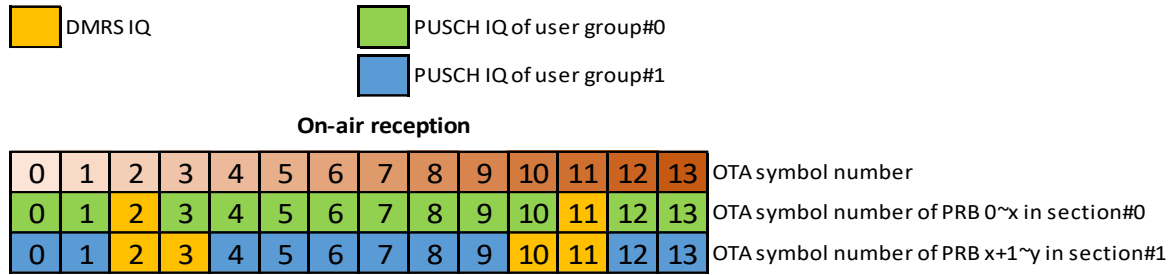
Figure 7.7.25.2-1: On-air symbol reception
