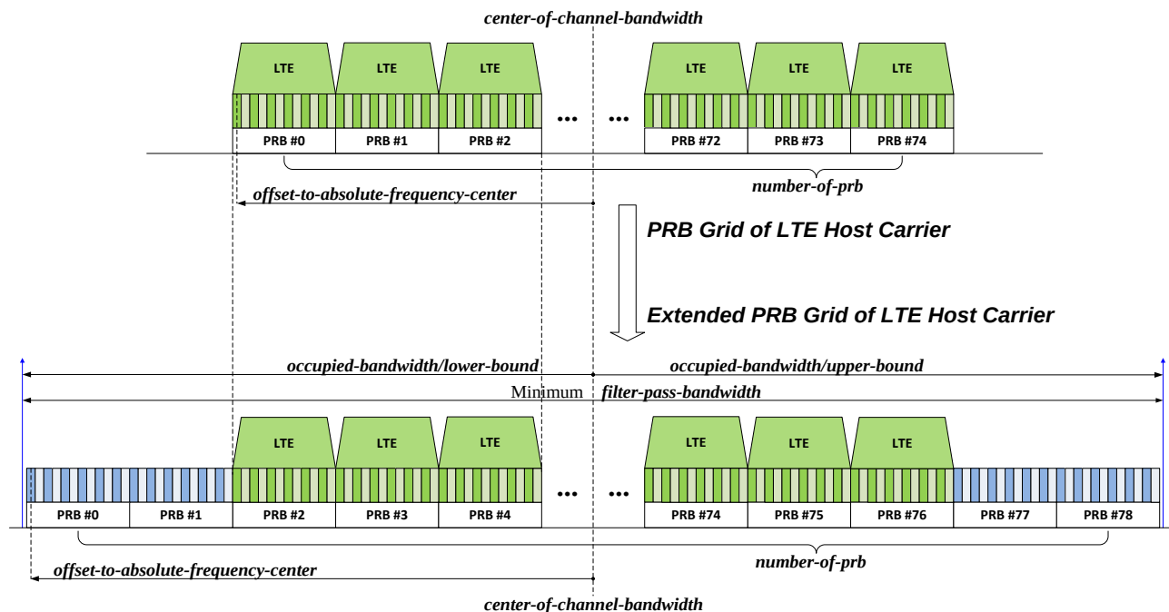
Figure 15.4.3-1: Example of extended PRB grid (UL)
