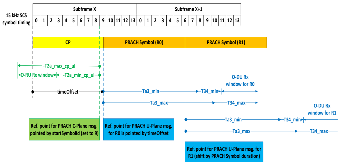
Figure 4.4.3-4: Timing relations for PRACH (Example 2: PRACH Format 1)
