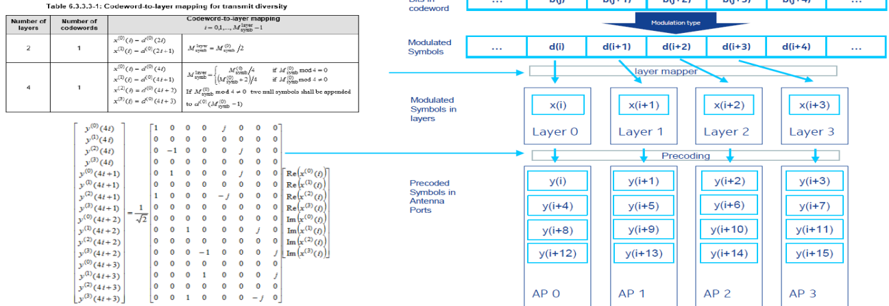
Figure I.3-1: Case 3 Layer Mapping
