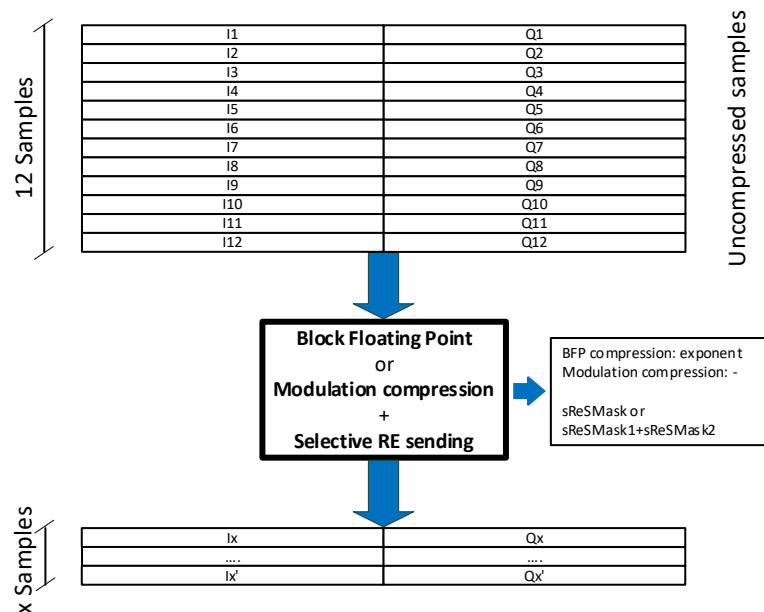
Figure A.6.1-1: Selective RE sending Compression data representation
