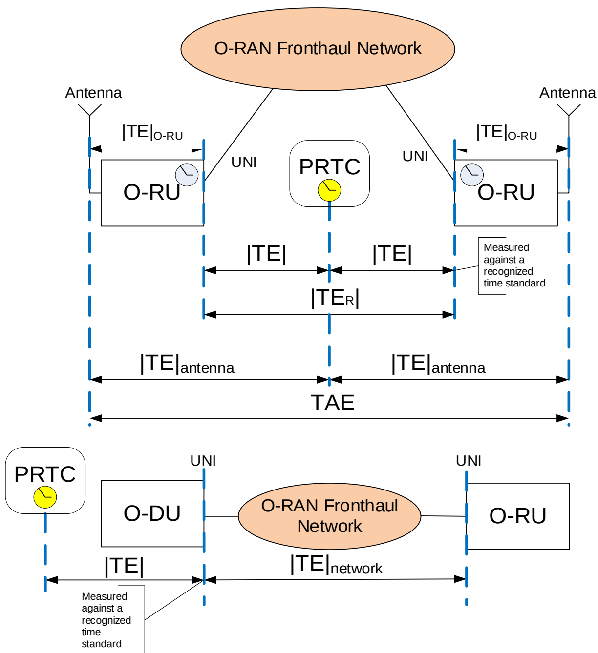
Figure 11.2.5.5-1: Definition of |TE| and TAE and UNI
