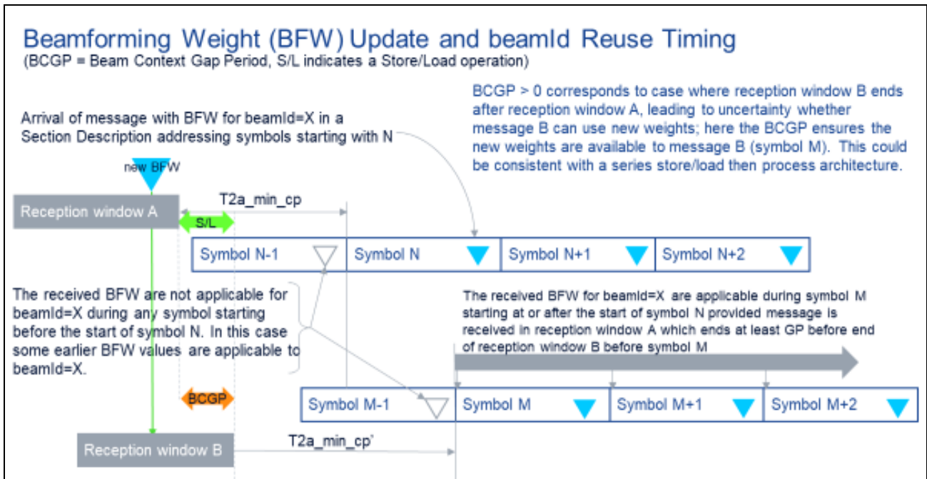
Figure 12.4.3.2-1: BFW Update Example #1 using beam-context-gap-period
