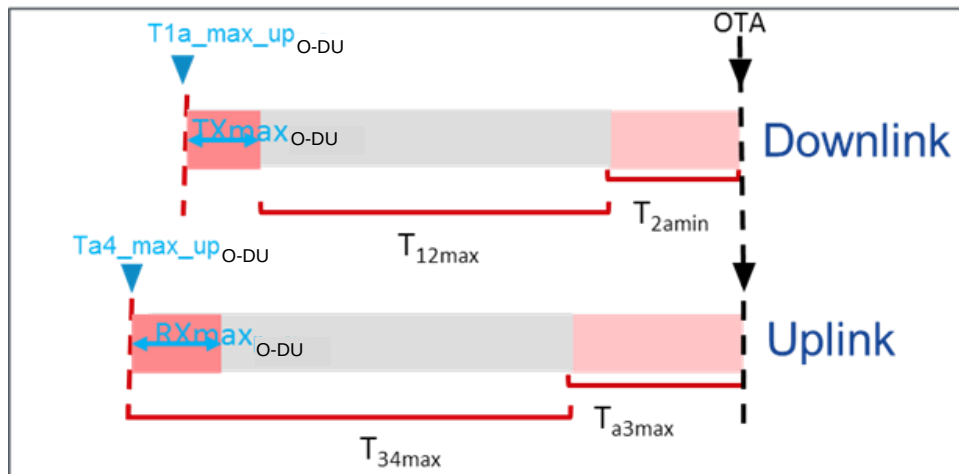
Figure 4.4.5-1: Uplink and downlink timing parameter relationship
