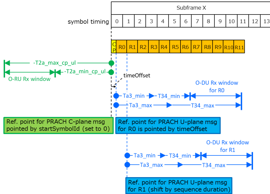
Figure 4.4.3-5: Timing relations for PRACH (Example 3: PRACH Format B4)
