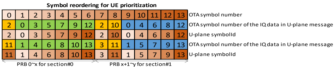
Figure 7.7.25.3-2: A UE prioritization use case of per-section tx-window reassignment method
