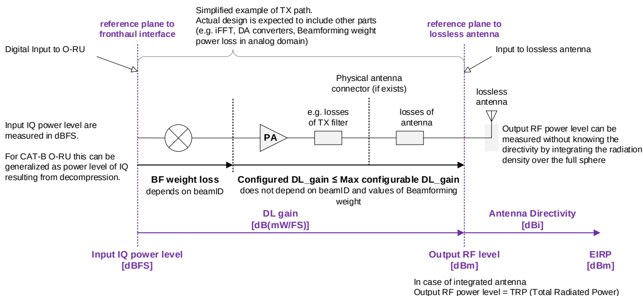
Figure 8.1.3.2.1-2: Details of DL gain
