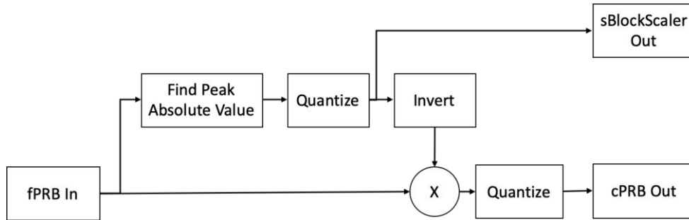
Figure A.2.1-1: Block scaling compression process diagram
