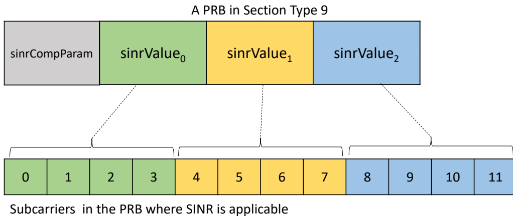
Figure 7.2.11-5: Example 11 of SINR reporting in Section Type 9 with sinr-per-prb = 3
