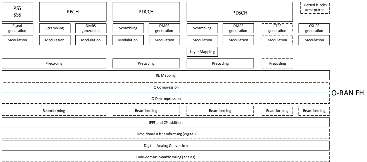
Figure 4.2.2.1-3: Lower layer DL split description, NR, Category A Radio
