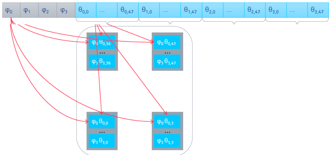
Figure K.3-1: Use case B
