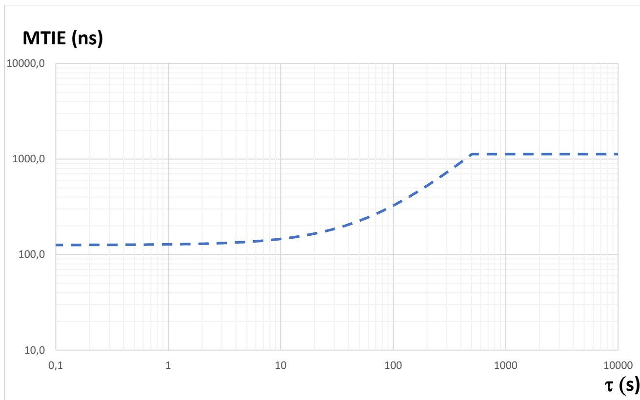
Figure H.2.5-1: MTIE limit at the input to an O-RU in LLS-C3
