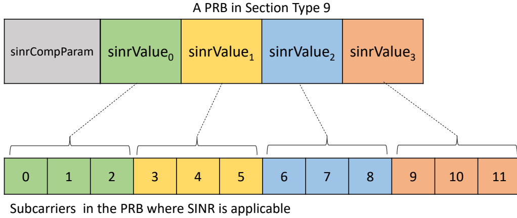
Figure 7.2.11-6: Example 12 of SINR reporting in Section Type 9 with \text{sinr-per-prb} = 4
