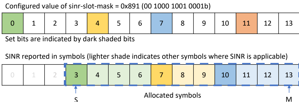
Figure 7.2.11-4: Example 7 of SINR reporting in Section Type 9 with \text{sinr-slot-mask} = 0x891 and allocation spanning symbols 3 to 13
