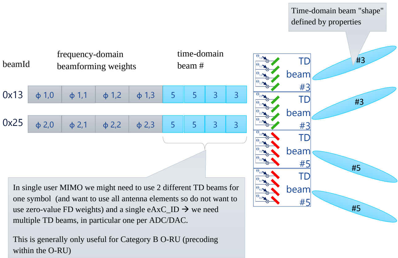
Figure 12.4.3.4.3-1: Example of updatable-weight frequency-domain plus fixed time-domain beamforming
