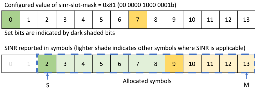
Figure 7.2.11-3: Example 6 of SINR reporting in Section Type 9 with \text{sinr-slot-mask} = 0x81 and allocation spanning symbols 2 to 13
