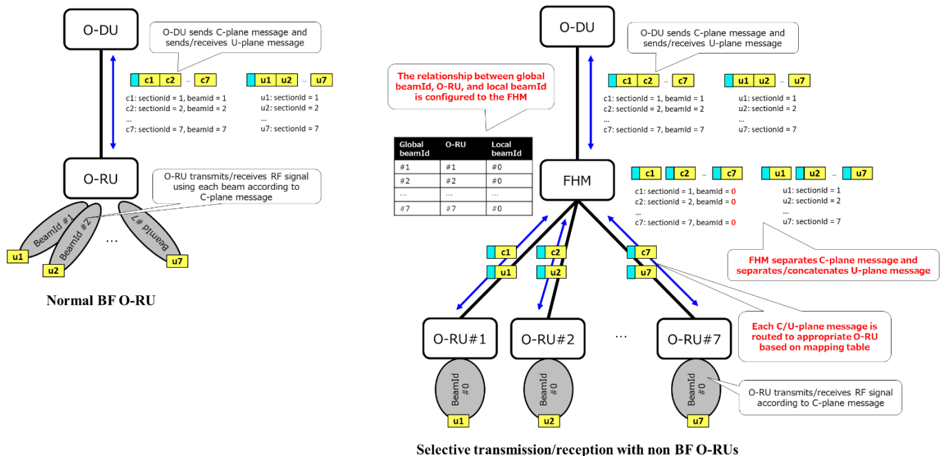
Figure M.2-1: C/U-Plane processing and RF signal transmission/reception procedure comparison (non BF O-RU case)
