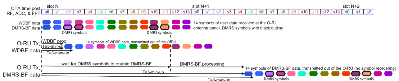
Figure 12.6.1.4-1: Comparison of WDBF delay profile versus DMRS-BF delay profile
