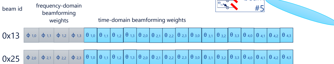
Figure 12.4.3.4.2-1: Example of updatable-weight frequency-domain and time-domain beamforming
