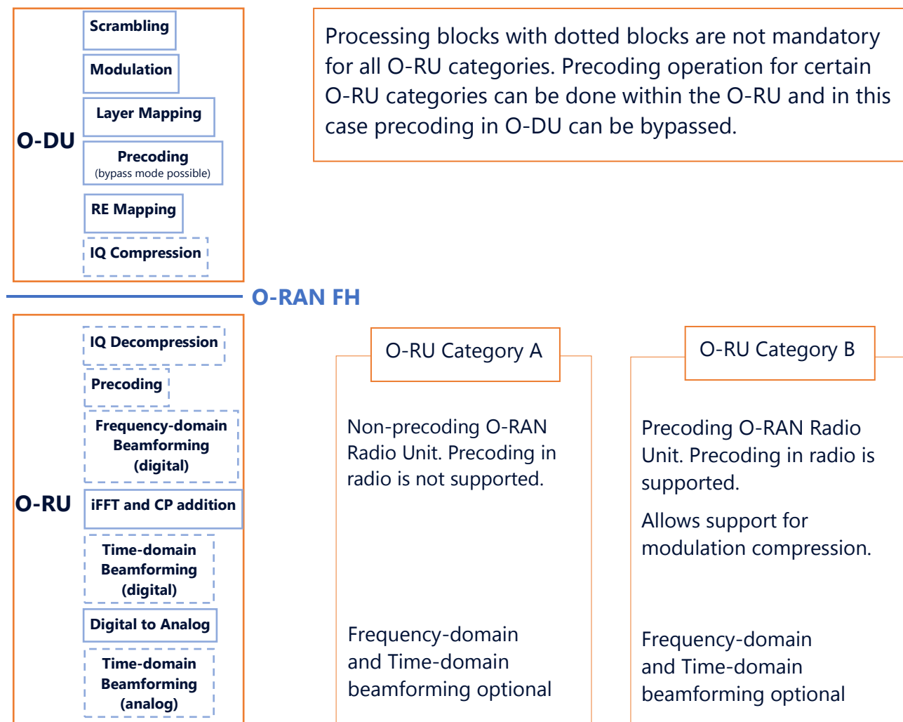
Figure 4.2.1-1: Split Point and Category A and Category B O-RAN Radio Units
