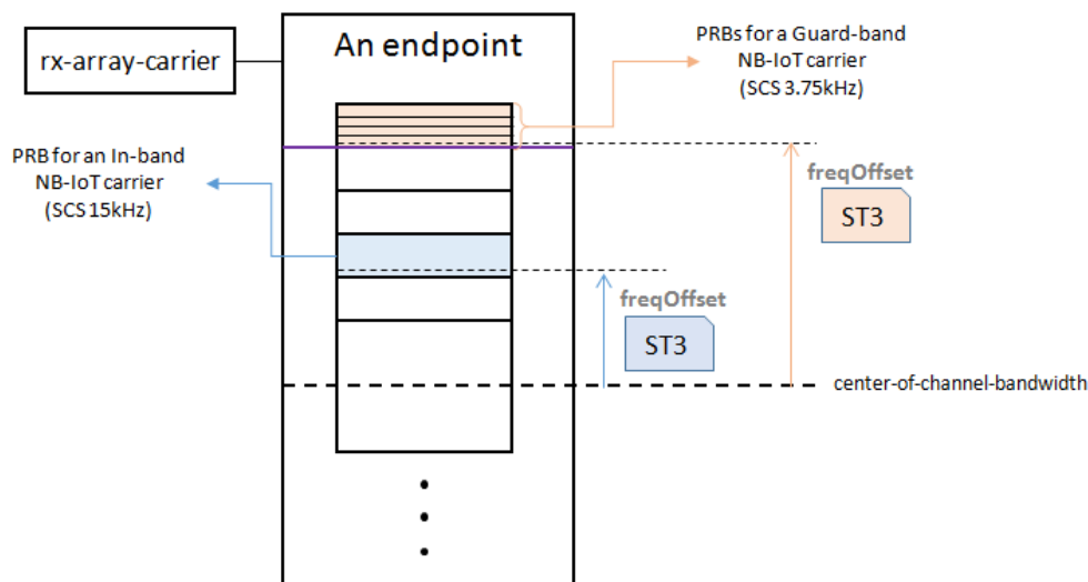
Figure 15.5.2-1: Example for SSSC method to indicate SCSs 3.75 kHz and 15 kHz of NPUSCH using ST 3
