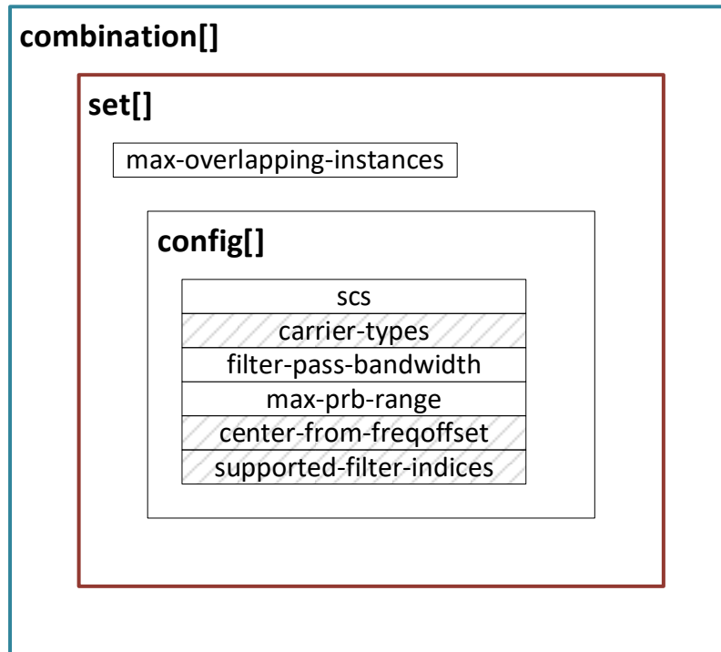
Figure 15.9-1: Supported configuration combinations group list overview
