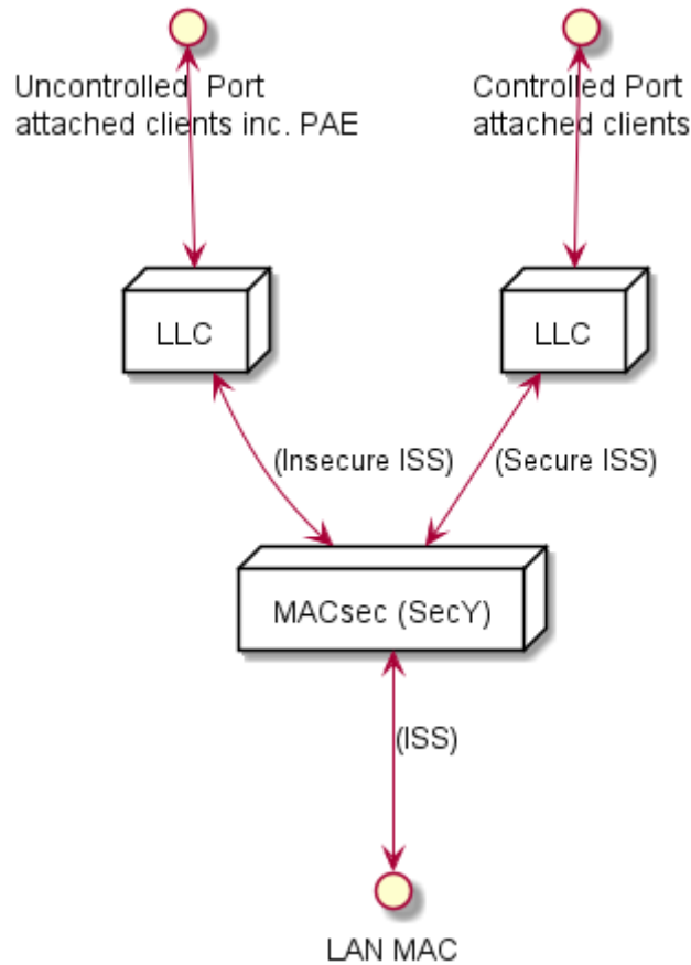
Figure 7.13.4.-1: Simultaneous access to controlled and un-controlled ports.
