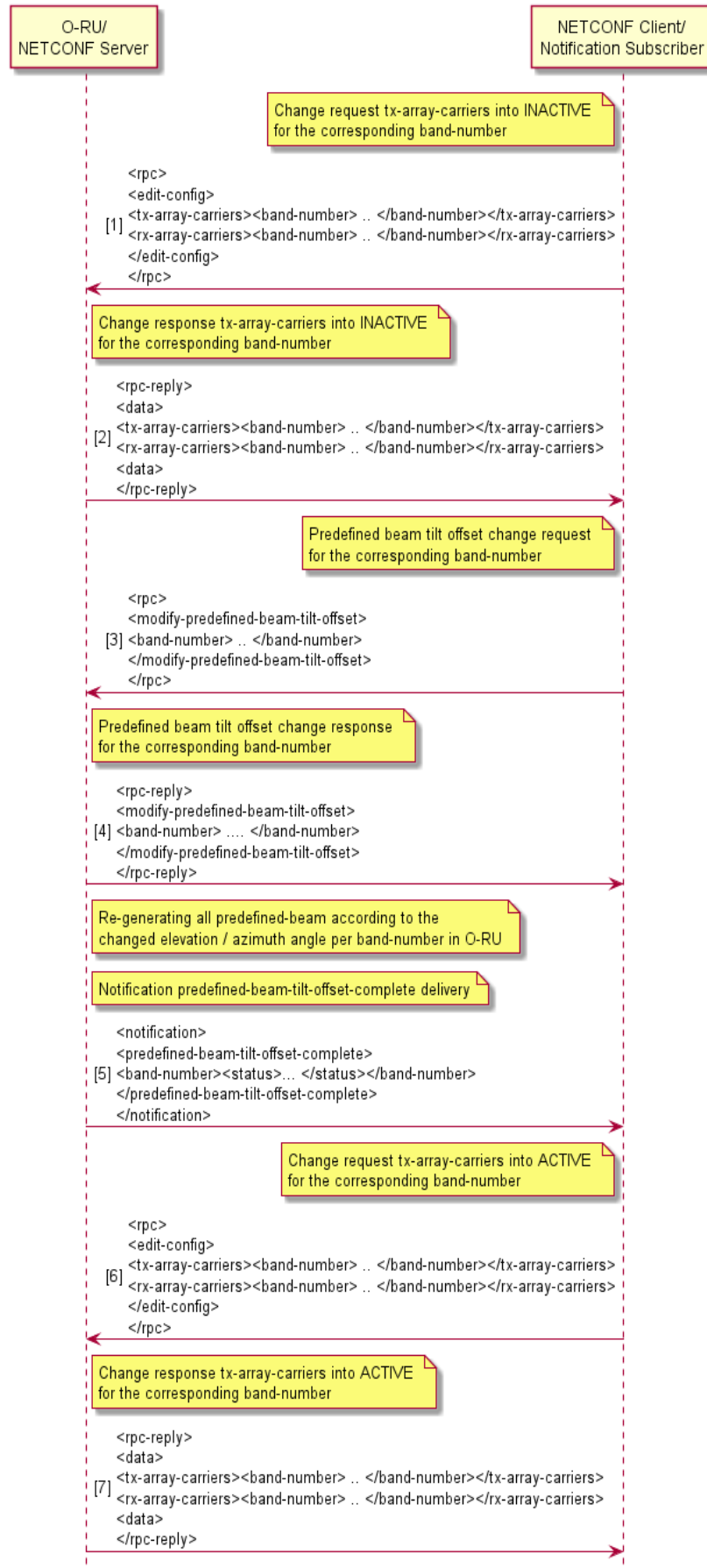
Figure 15.4.4-2: Procedure for the predefined-beam-tilt-offset
