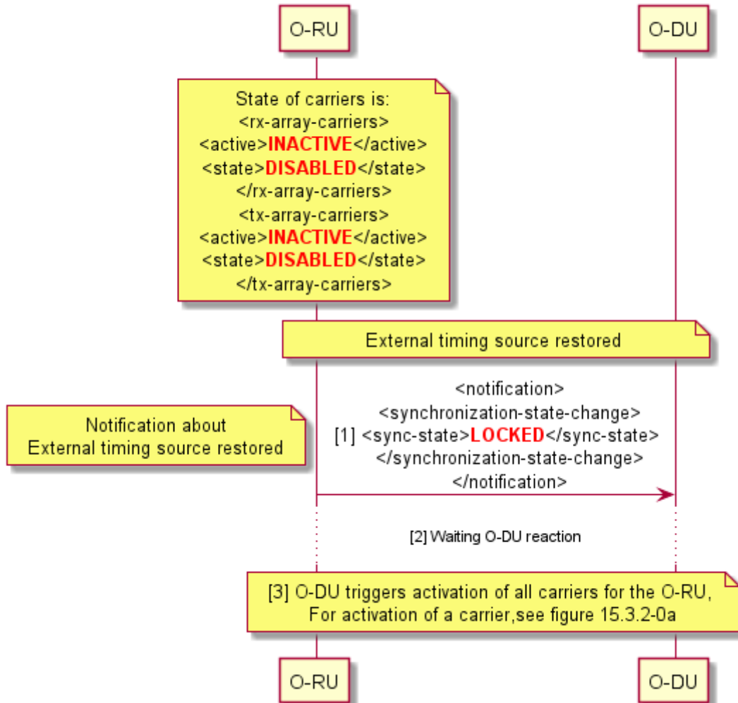
Figure 15.3.3.3-1: Synchronisation restored and carrier reactivation scenario
