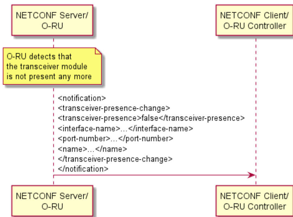
Figure 7.2.2-1: Transceiver presence change notification
