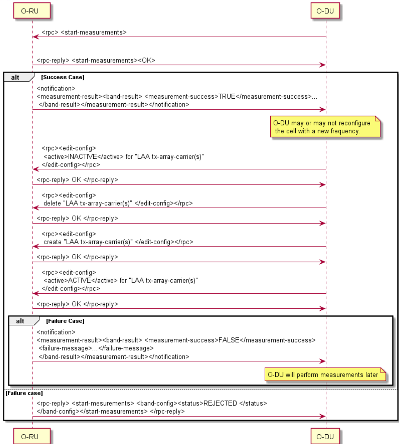
Figure 16.1-1: Carrier-Selection Call-flow
