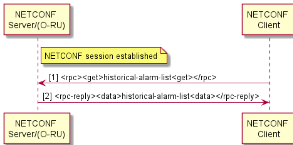
Figure 11.6-1: Read Historical Alarms
