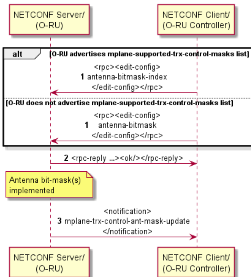
Figure 20.3.2.3-1 – TRX control configuration (M-Plane controlled)
