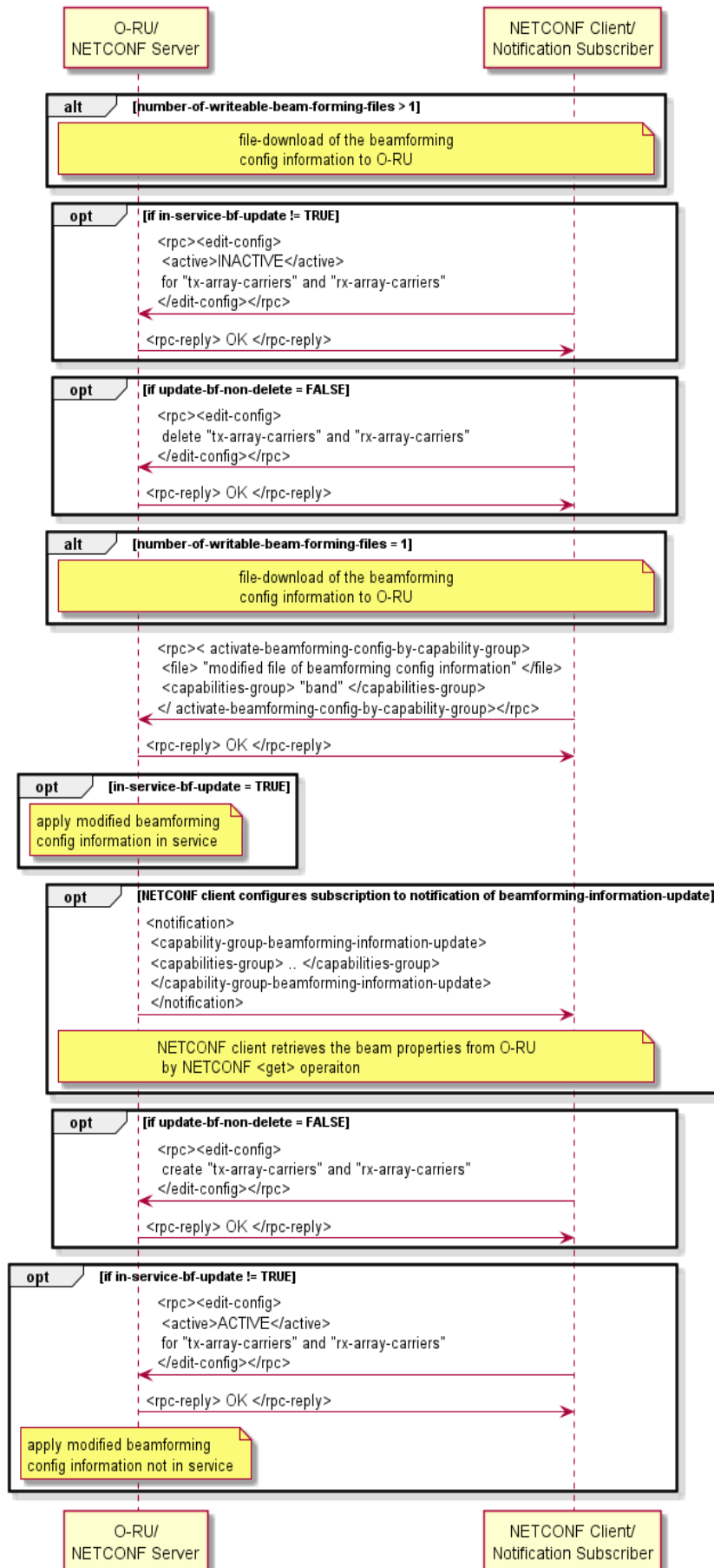
Figure 15.4.3-2: Method to Apply the modified file for Beamforming Configuration Information
