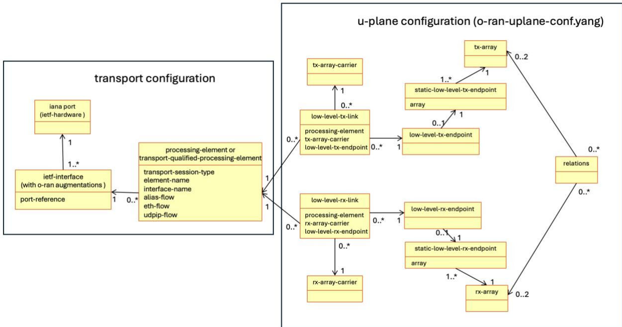
Figure 15.2.4-1: Diagram showing relations between CU-Plane and carrier management elements
