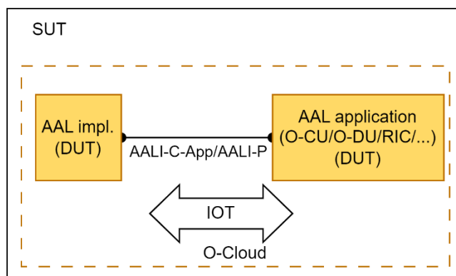
Figure 4.1-3: SUT configurations for AALI IOT(AALI-C-App/AALI-P)
