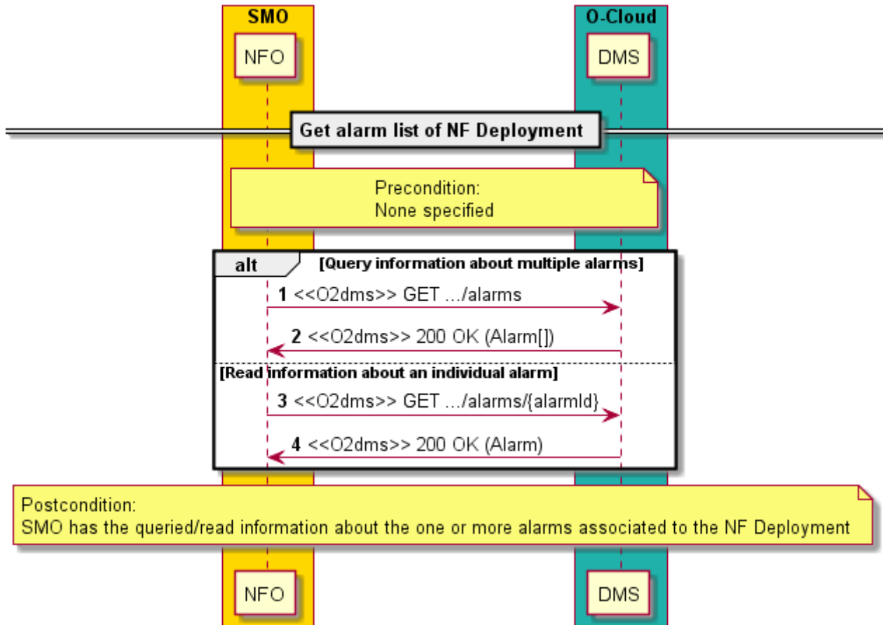
Figure 2.4.3.1-1: Flow of get alarm list of NF Deployment
