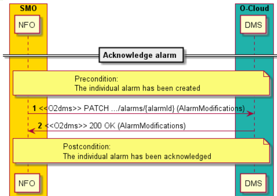
Figure 2.4.3.3-1: Flow of acknowledging alarm of NF Deployment
