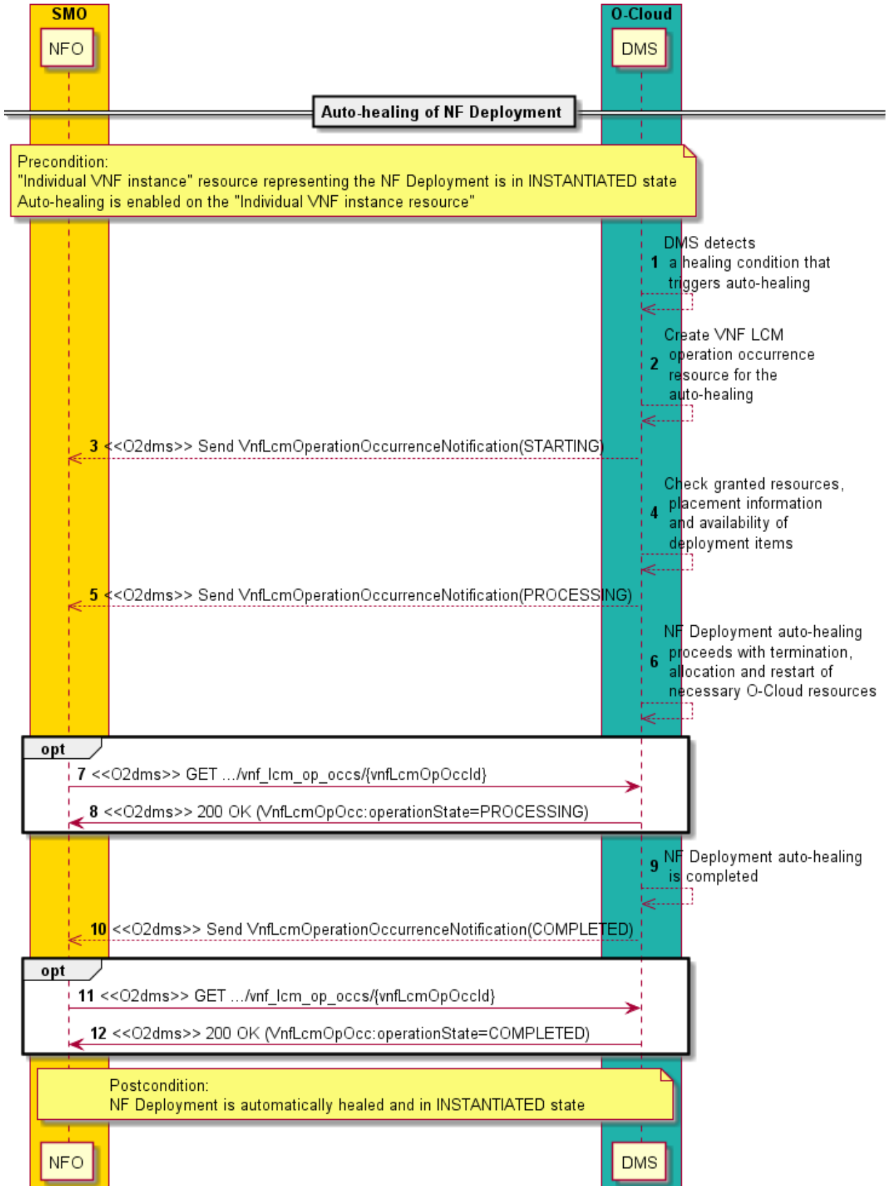
Figure 2.4.2.4.3-1: Flow of NF Deployment auto-healing
