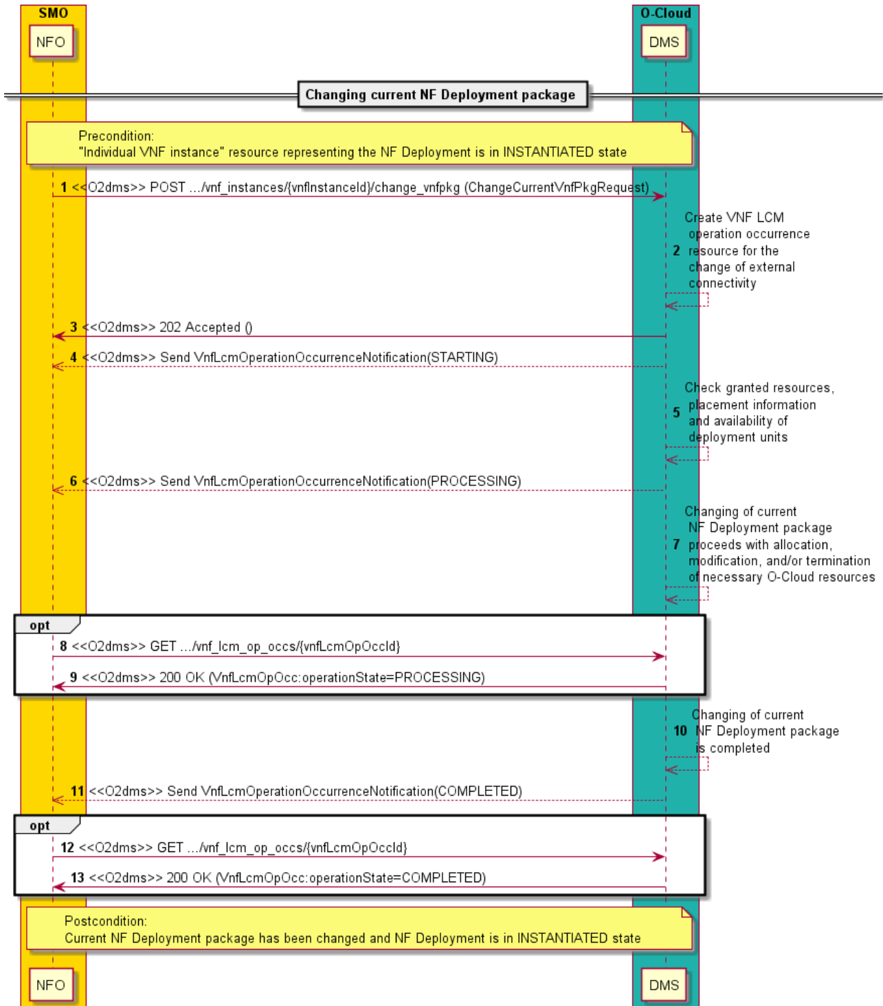
Figure 2.4.2.7-1: Flow of changing current NF Deployment package
