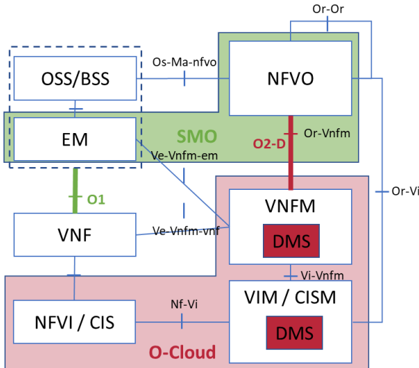
Figure 2.1-1: Representation of "O2-D demarcation #1".
