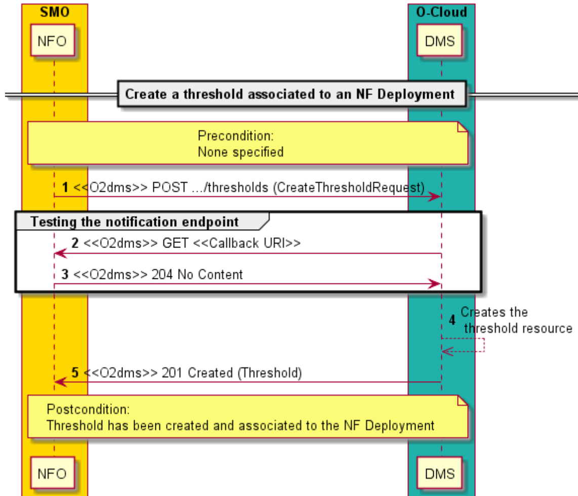
Figure 2.4.4.4-1: Flow of creating a threshold associated to an NF Deployment
