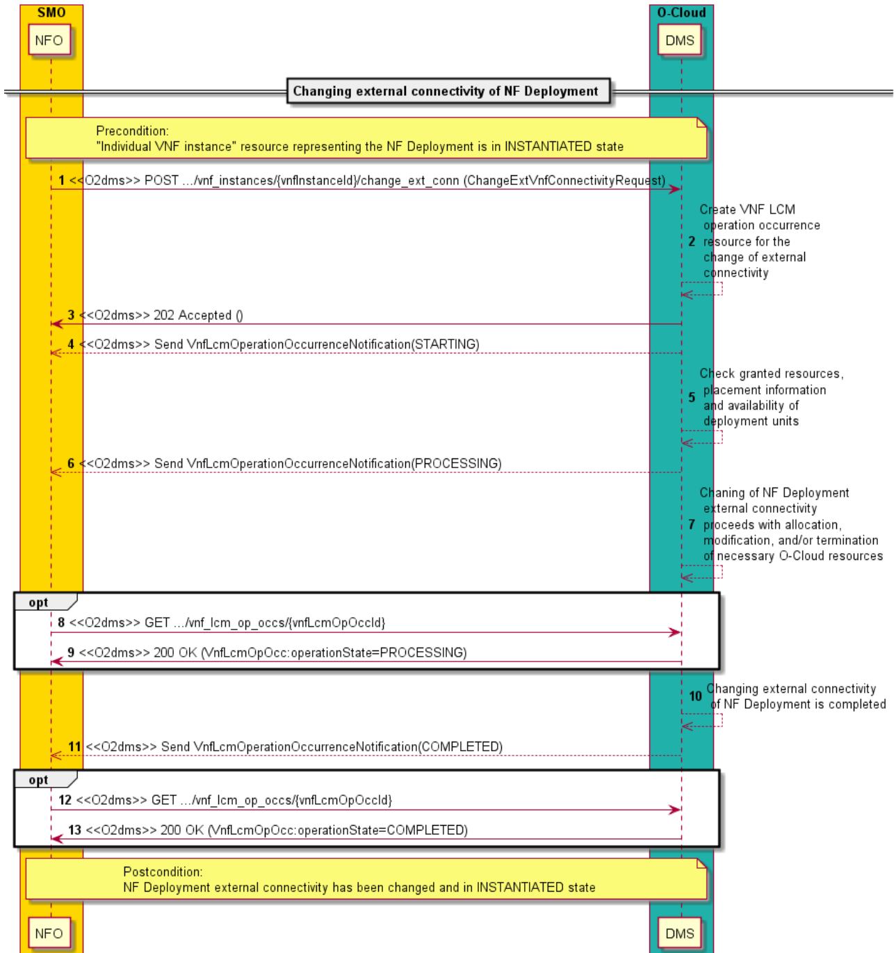
Figure 2.4.2.6-1: Flow of changing external connectivity of NF Deployment
