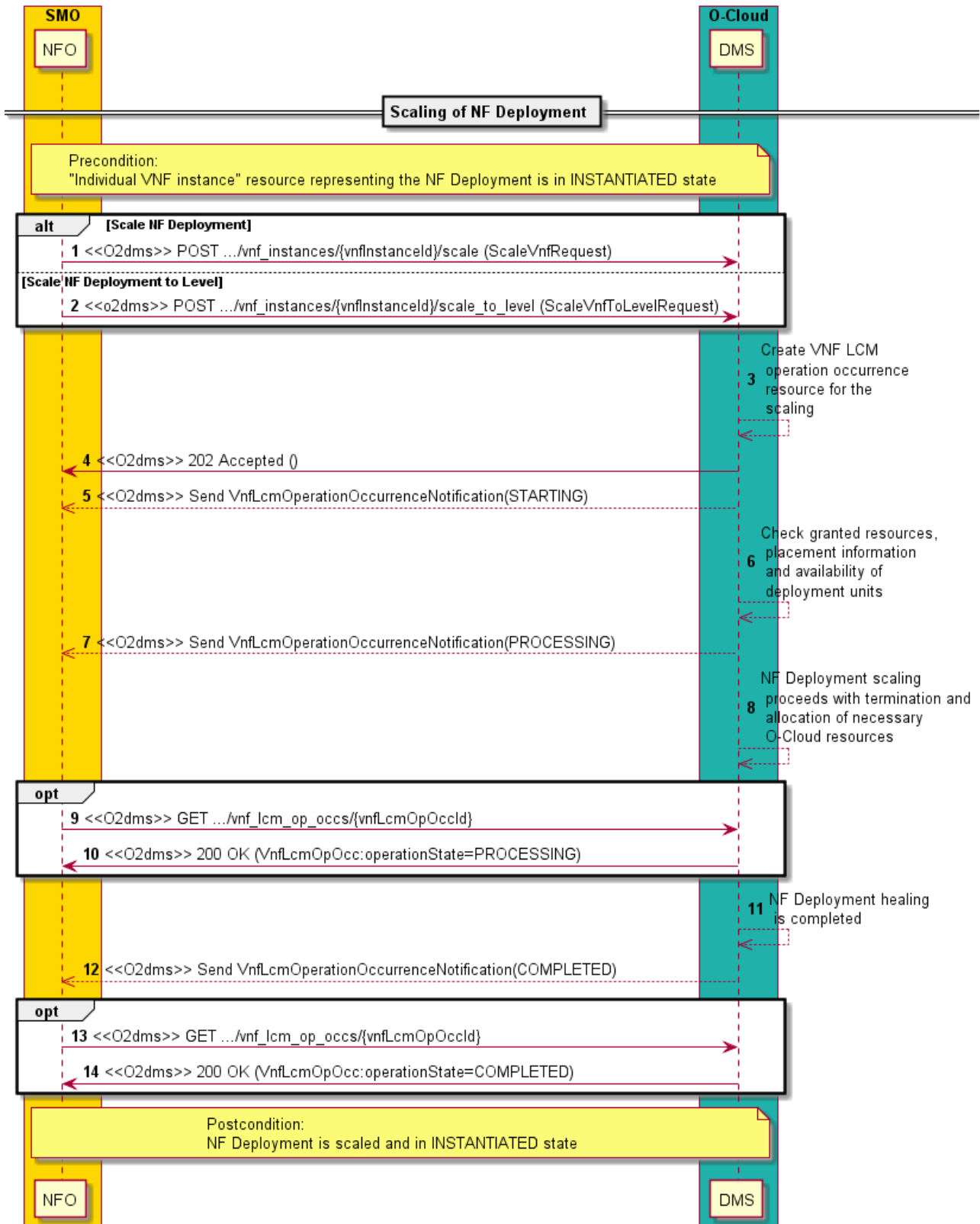
Figure 2.4.2.5.2-1: Flow of NF Deployment scaling based on management request
