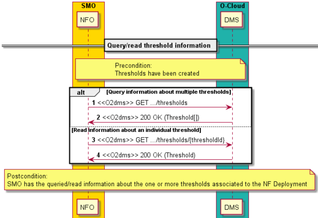
Figure 2.4.4.5-1: Flow of query/reading information of thresholds associated to an NF Deployment
