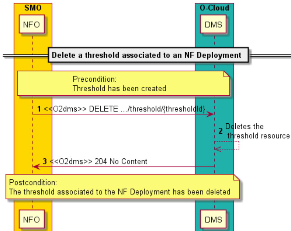
Figure 2.4.4.6-1: Flow of deleting a threshold associated to an NF Deployment
