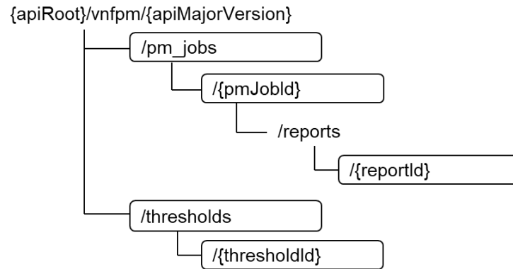
Figure 3.4.3-1: Resource URI structure of the O2dms_DeploymentPerformance Service API
