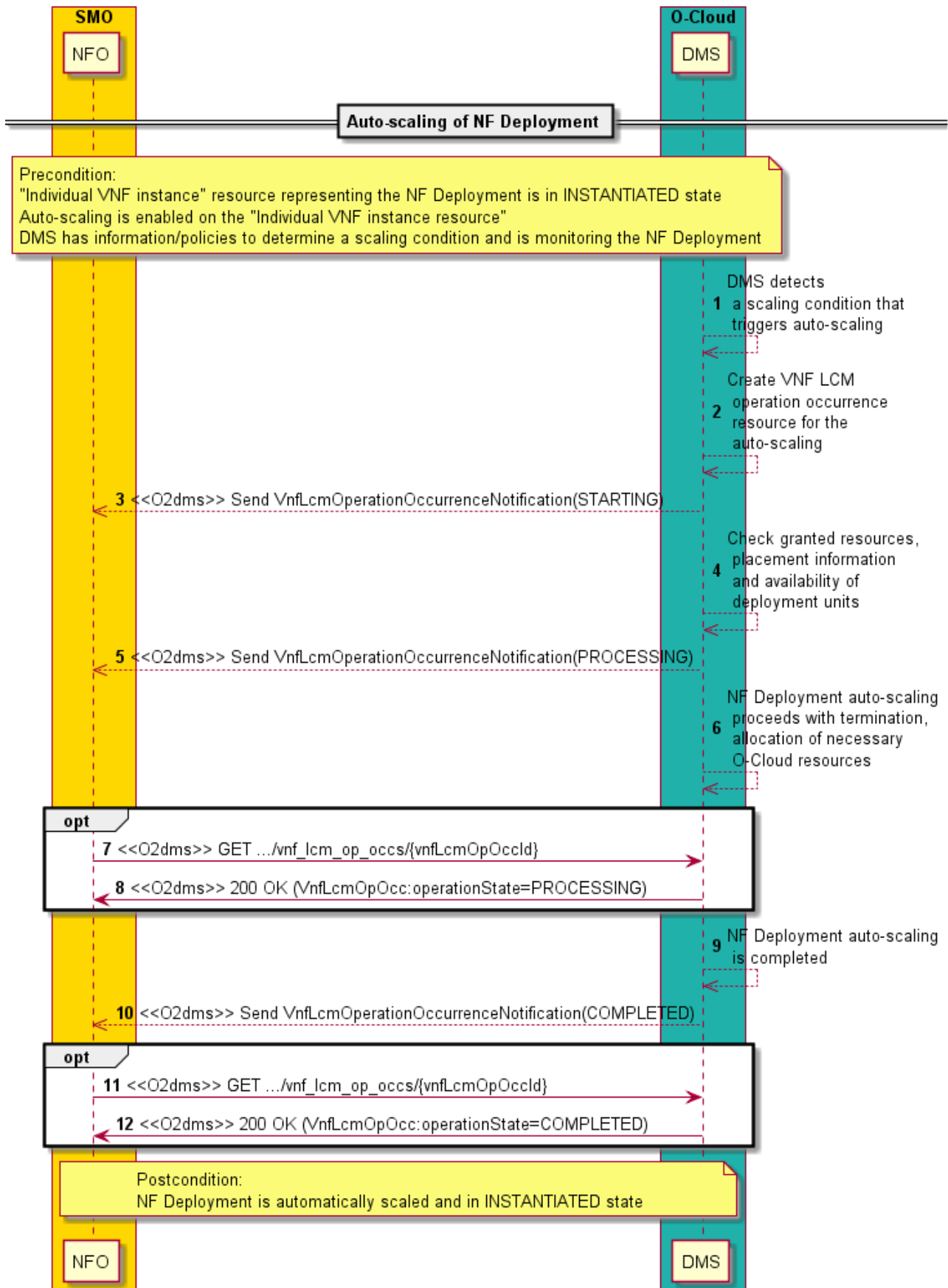
Figure 2.4.2.5.3-1: Flow of NF Deployment auto-scaling
