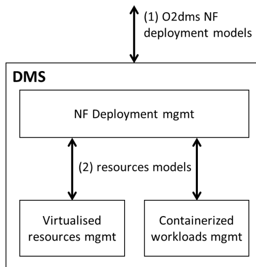
Figure 2.5.7.2-1: Models in interactions
