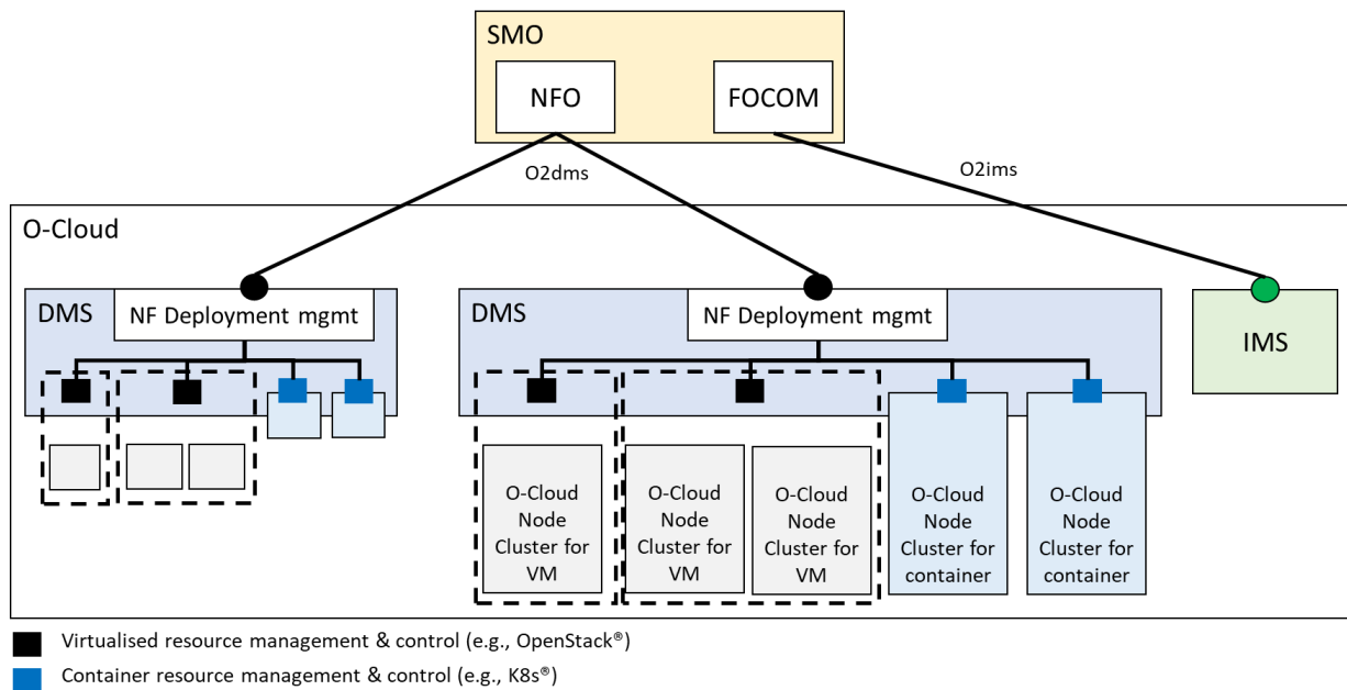
Figure 2.5.1-1: Exemplary configuration of O-Cloud and DMS relationship with O-Cloud Node Clusters
