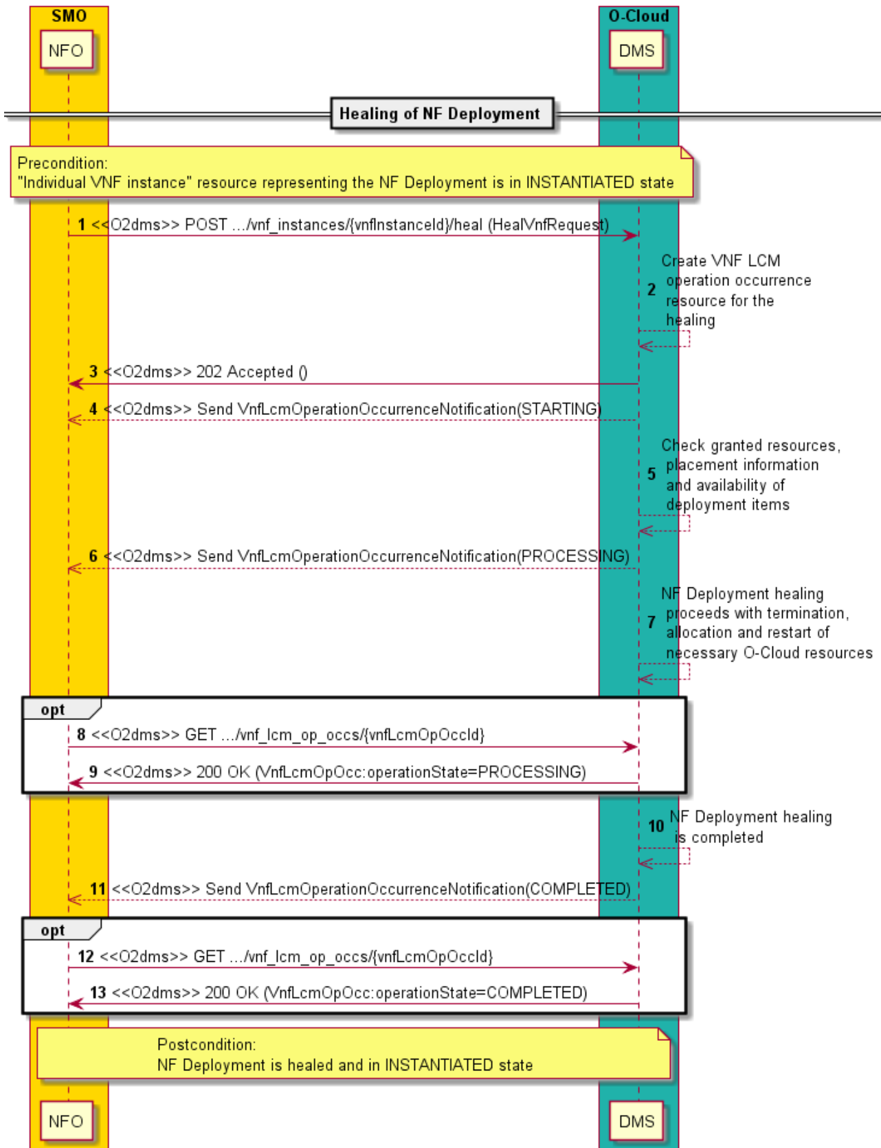
Figure 2.4.2.4.2-1: Flow of on-demand NF Deployment healing
