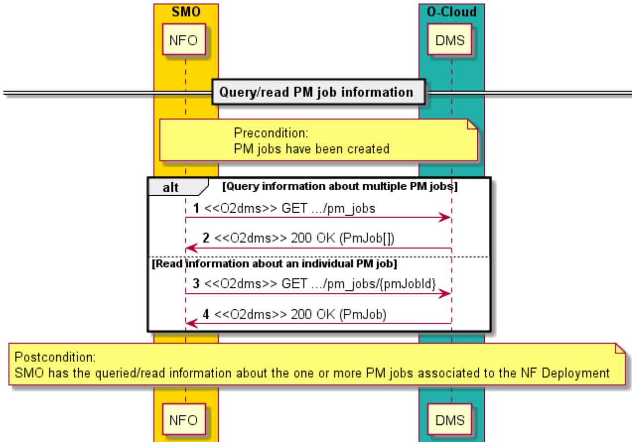
Figure 2.4.4.2-1: Flow of query/reading information of PM jobs associated to an NF Deployment
