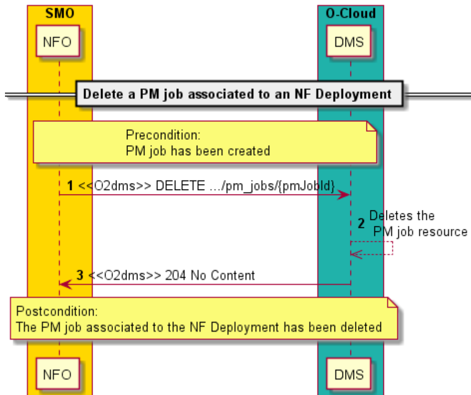
Figure 2.4.4.3-1: Flow of deleting a PM job associated to an NF Deployment
