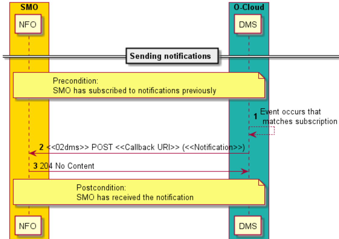
Figure 2.4.3.2-1: Flow of fault management notifications associated to an NF Deployment
