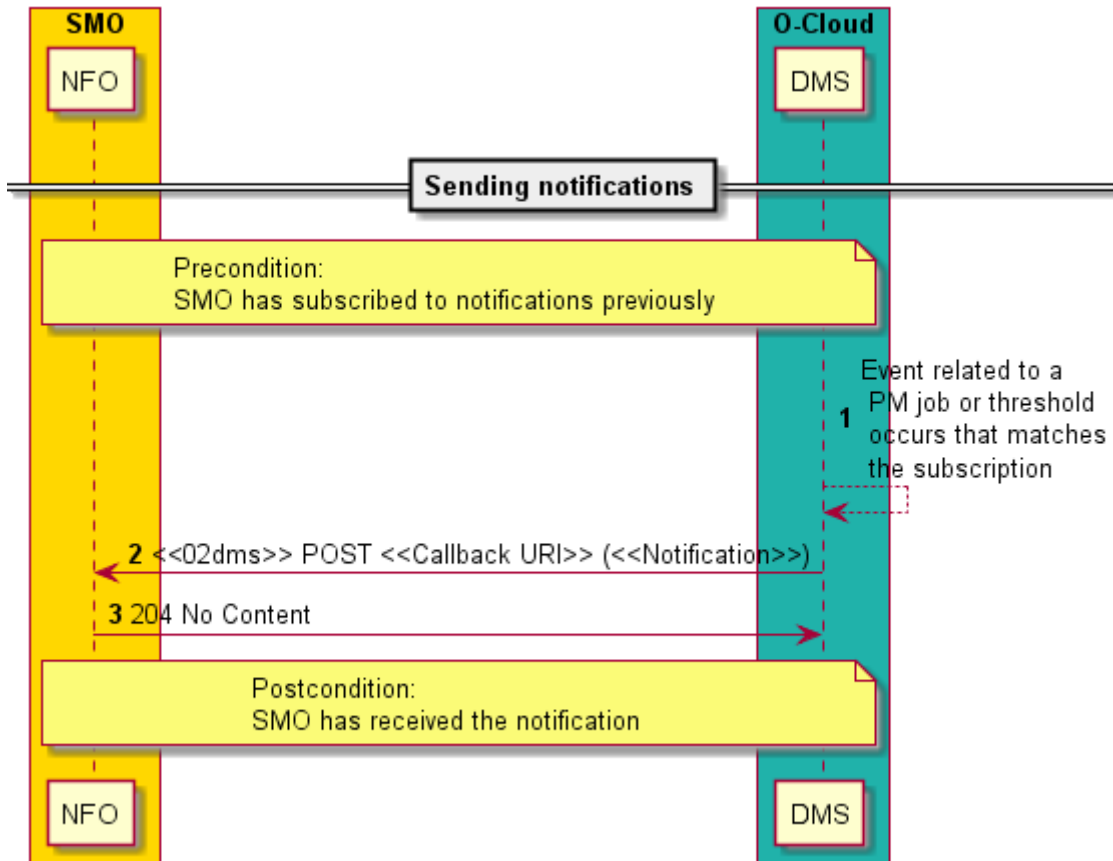
Figure 2.4.4.7-1: Flow of performance management notifications associated to an NF Deployment
