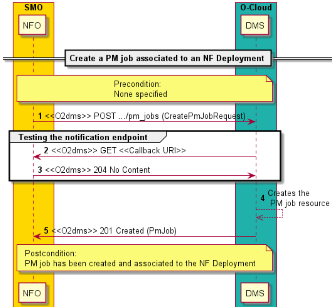
Figure 2.4.4.1-1: Flow of creating a PM job associated to an NF Deployment
