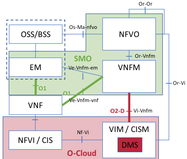
Figure 2.1-2: Representation of "O2-D demarcation #2".
