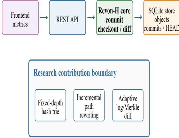
Fig. 1. Revon system architecture and the boundary of its research contribution.
