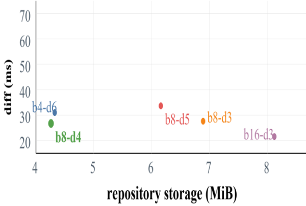
Fig. 6. Fixed-trie sensitivity; dots show median diff latency, and the axis extends above the largest measured p75.
