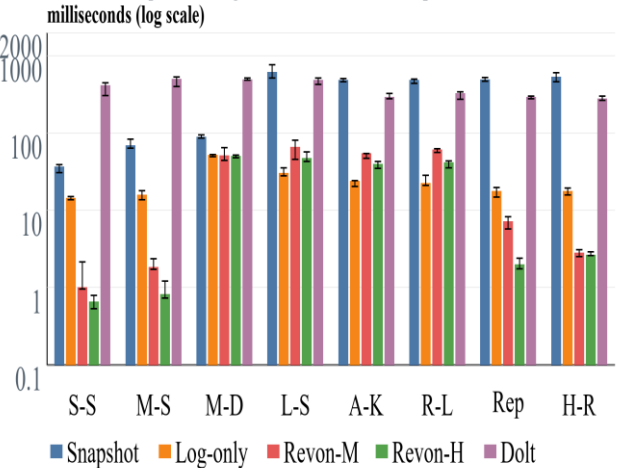
Fig. 4. Diff latency across eight scenarios, including separate application-key, range, repeated-key, and hash-route update locality; lower is better.
