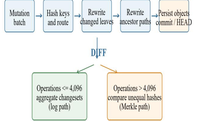
Fig. 2. Incremental commit path and adaptive diff decision.
