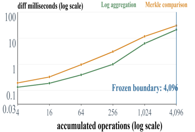
Fig. 3. Independent threshold calibration; 4,096 is the largest sampled log-favorable point.
