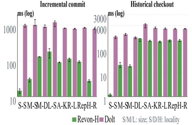
Fig. 5. Revon-H and Dolt operational latency; lower is better.
