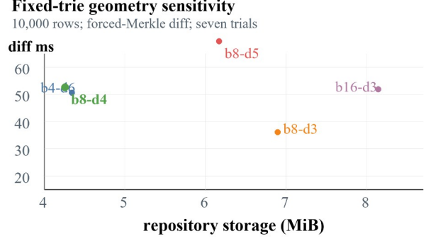
Fig. 6. Fixed-trie sensitivity; points show median diff latency, and the axis extends beyond the largest measured 75th percentile.
