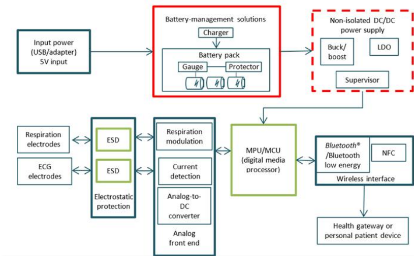
Figure 5.1: Hardware Subsystem Block Diagram (Power Management, Analog Front-End, Host MCU & Bluetooth Telemetry).
