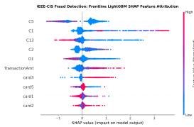
Figure 2: TreeSHAP Global Feature Attribution Summary on IEEE-CIS Benchmark ( N = 118,108 ).
