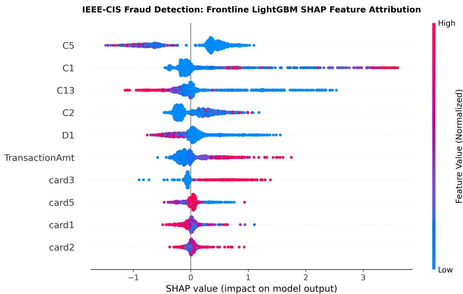
Figure 2: Frontline Model Global TreeSHAP Feature Attribution Summary ( N = 118,108 Transactions).
