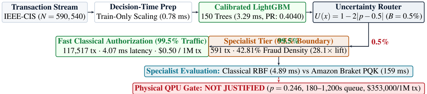
Figure 1: Asymmetric Hybrid Fraud Detection Architecture. Frontline calibrated detector authorizes 99.5% of traffic at 4.07 ms latency. Only the 0.5% boundary transactions are escalated to specialist analysis, isolating quantum latency and costs.
