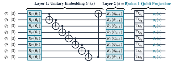
Figure 1: 8-Qubit Amazon Braket Quantum Circuit and Projection Schematic (Typeset via TikZ) . Scaled PCA features parametrize single-qubit R_Y gates coupled via circular CNOT entanglement ladder ( d = 2 ). The state is projected onto 1-qubit reduced density operators \rho_i(x) .
