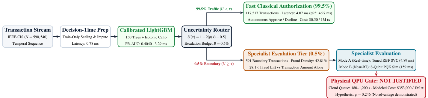
Figure 1: Asymmetric Hybrid Fraud Detection Architecture (Typeset via TikZ). The frontline calibrated detector authorizes 99.5% of traffic at 4.07 ms latency. Only the 0.5% boundary transactions are escalated to specialist analysis, isolating quantum latency and operational costs.
