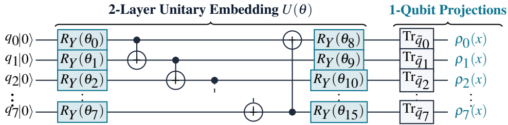
Figure 1: 8-Qubit Amazon Braket Quantum Circuit and Projection Schematic. Scaled PCA features parametrize single-qubit R_Y gates coupled via circular CNOT entanglement ladder ( d = 2 ). The state is projected onto 1-qubit reduced density operators \rho_i(x) .
