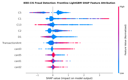
Figure 2: TreeSHAP Global Feature Attribution Summary on IEEE-CIS Benchmark ( N = 118,108 ).
