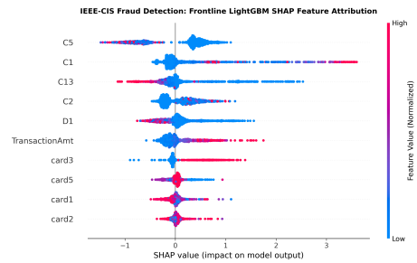
Figure 2: TreeSHAP Global Feature Attribution Summary on IEEE-CIS Benchmark. Attributions vary per transaction across =118,108, confirming absence of constant – feature artifacts.
