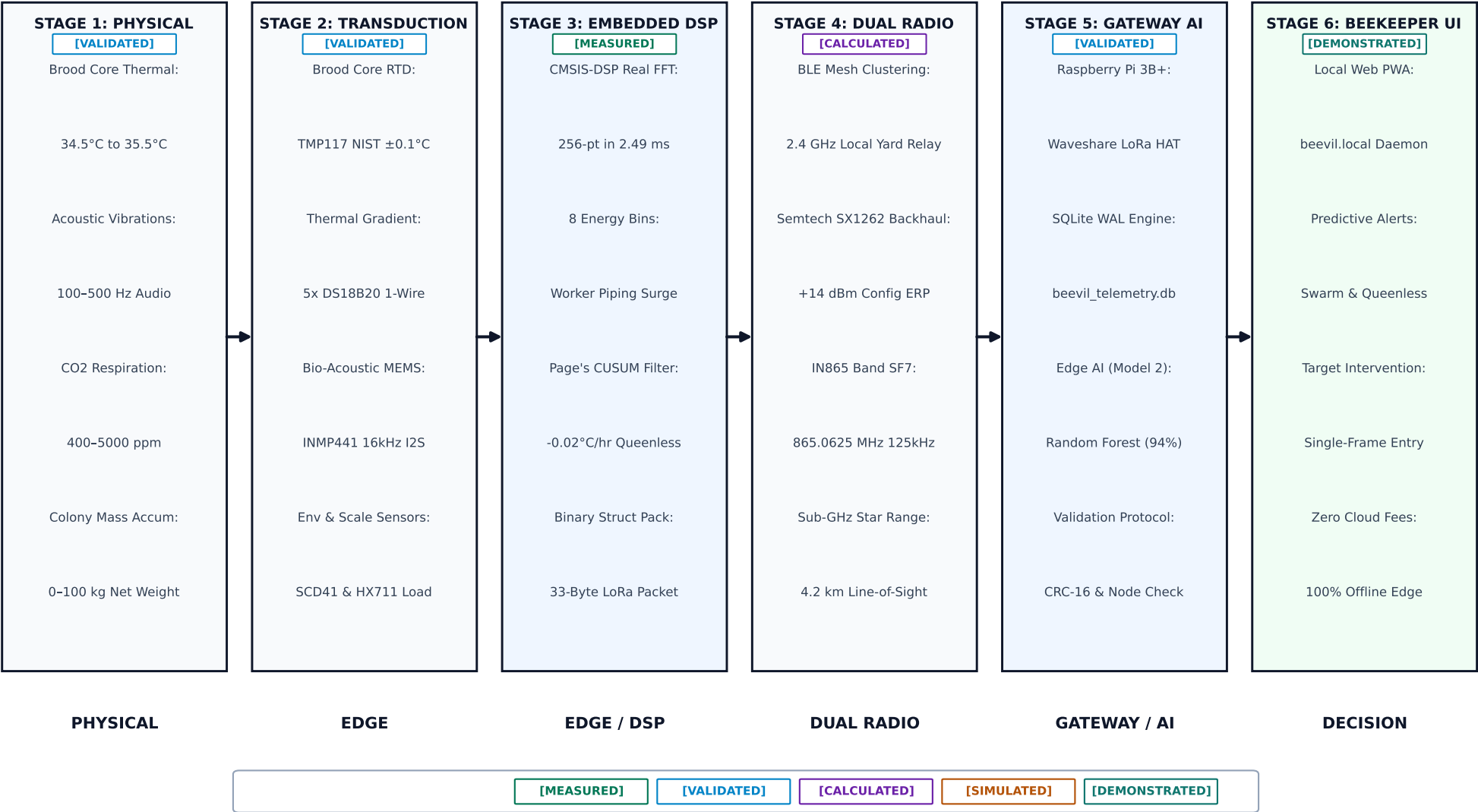
FIGURE 10: END-TO-END DATA FLOW PIPELINE Chronological 6-Stage Signal Transformation: Physical Phenomena to Beekeeper Decision [Video Frame Ready]
