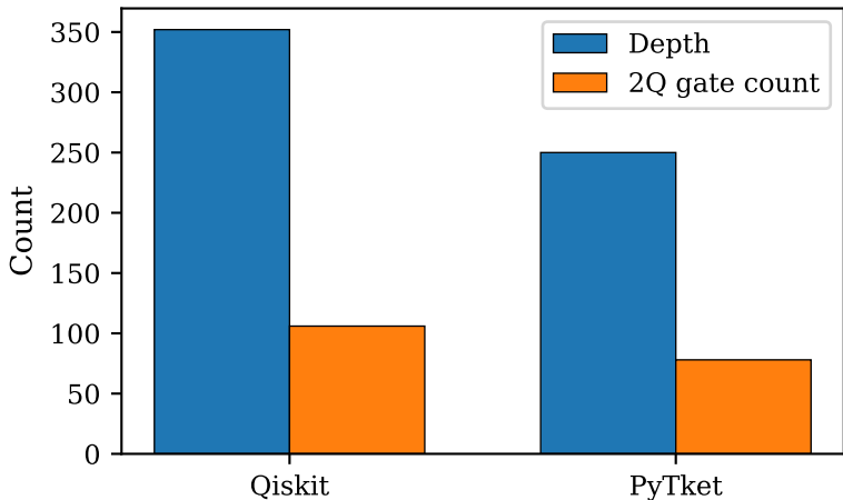
Post-routing circuit metrics (mean)
