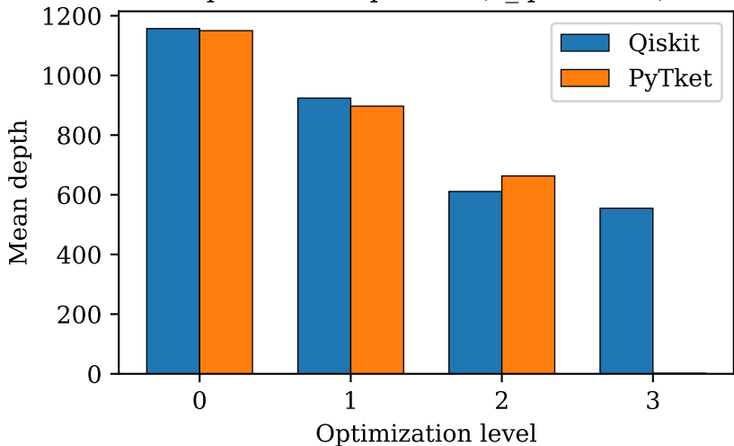
Opt-level comparison (n_qubits=10)
