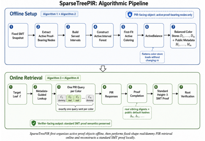
Fig. 3. SparseTreePIR algorithmic pipeline. Offline setup extracts active proof-bearing nodes, builds served intervals, colors the active interval forest, and balances color stores. Online retrieval uses public metadata to issue exactly one PIR query per color, then combines retrieved real sibling digests with public default hashes to reconstruct the standard height- h SMT proof.
