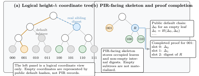
Fig. 2. Logical and retrieval views of an SMT. The verifier reasons about a complete height- h coordinate tree, but the PIR database should not store every empty coordinate. A membership proof is completed by combining PIR-retrieved non-default sibling digests with public default hashes.
