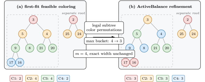
Fig. 5. Running example for the coloring stage. The first-fit feasibility stage leaves an uneven but valid split, while ActiveBalance applies accepted legal subtree recolorings and reaches a flatter partition on the same interval forest.
