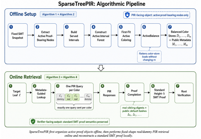
Fig. 3. SparseTreePIR algorithmic pipeline. Offline setup extracts active proof records, builds target-rank intervals, colors the laminar interval forest, and balances color subdatabases. Online retrieval uses public metadata to issue exactly one PIR query per color, then combines retrieved non-default sibling digests with public default hashes to reconstruct the standard height- h SMT proof.
