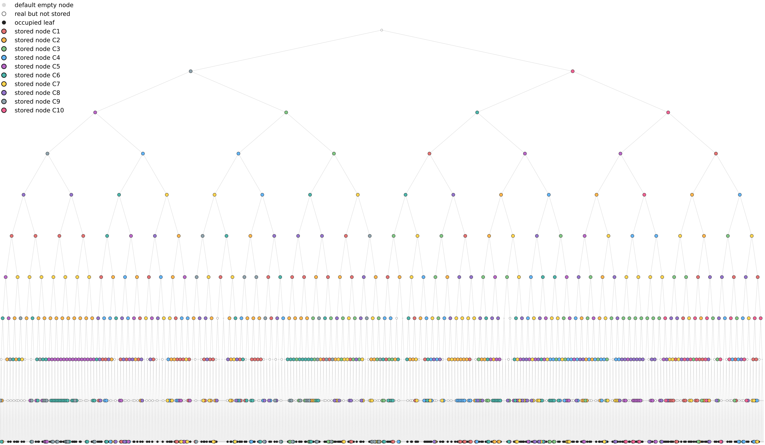
Complete Merkle tree (height 10) with stored proof-bearing nodes highlighted
