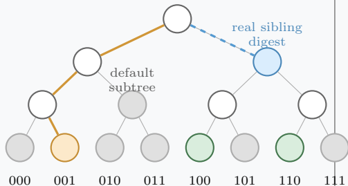
(a) Logical height- h coordinate tree
