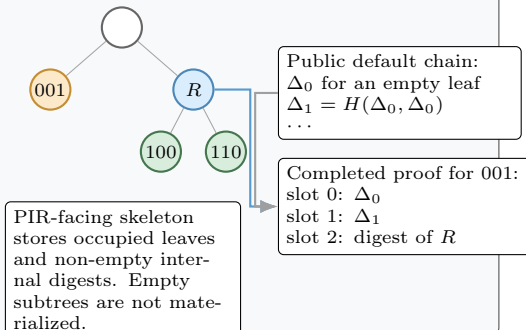
(b) PIR-facing skeleton and proof completion
