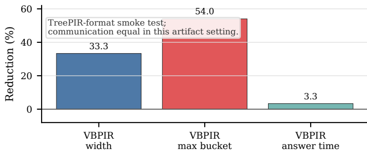
C. TreePIR artifact check: VBPIR TreePIR route vs VBPIR PBC route
